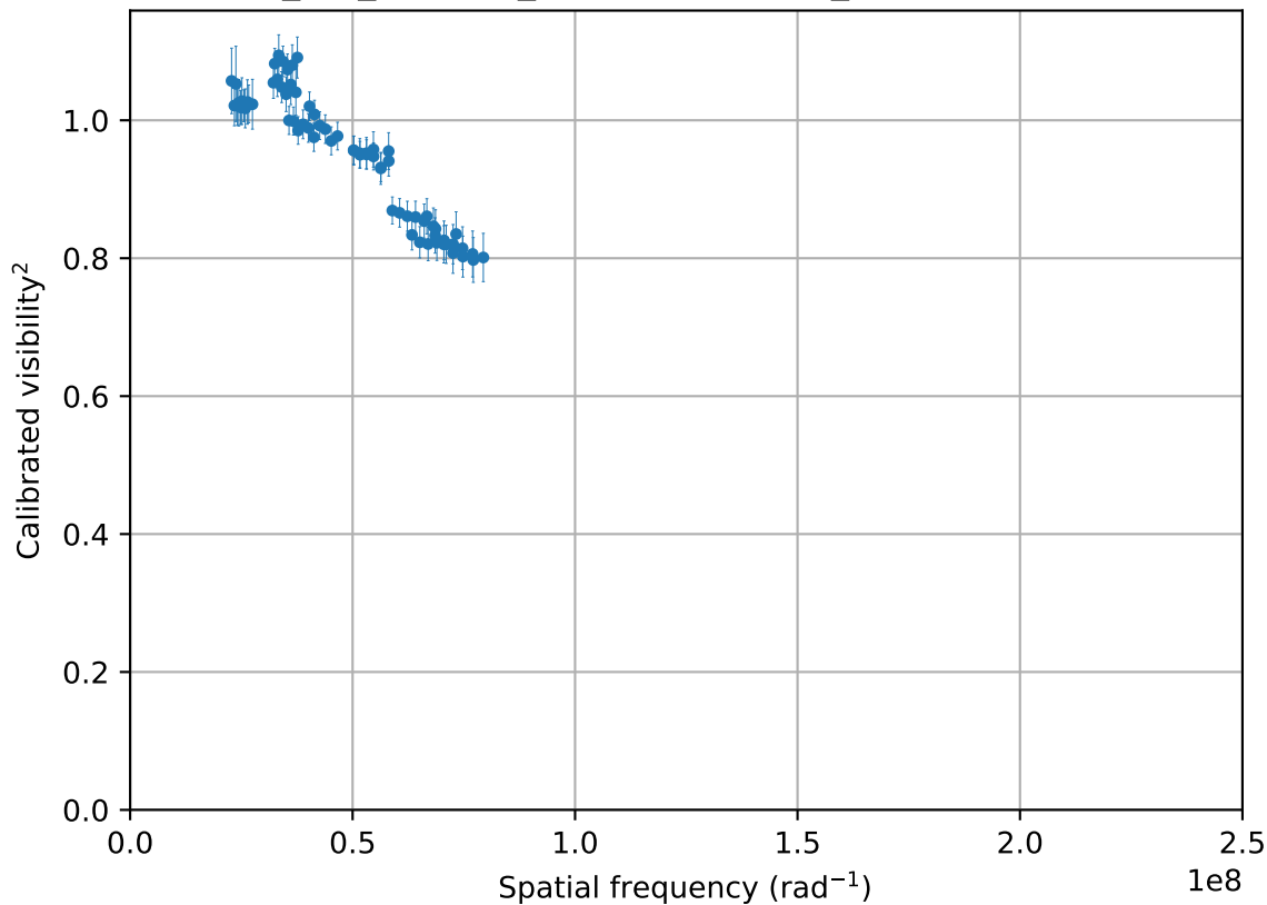
2019-11-25_SCI_HR2998_oidataCalibrated_499 (72 valid vis 2 points)
