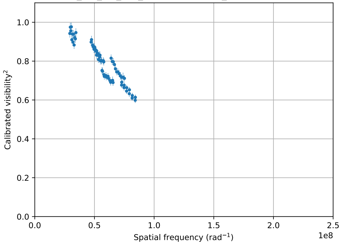
2019-11-27_SCI_zet_Tuc_oidataCalibrated_499 (72 valid vis 2 points)
