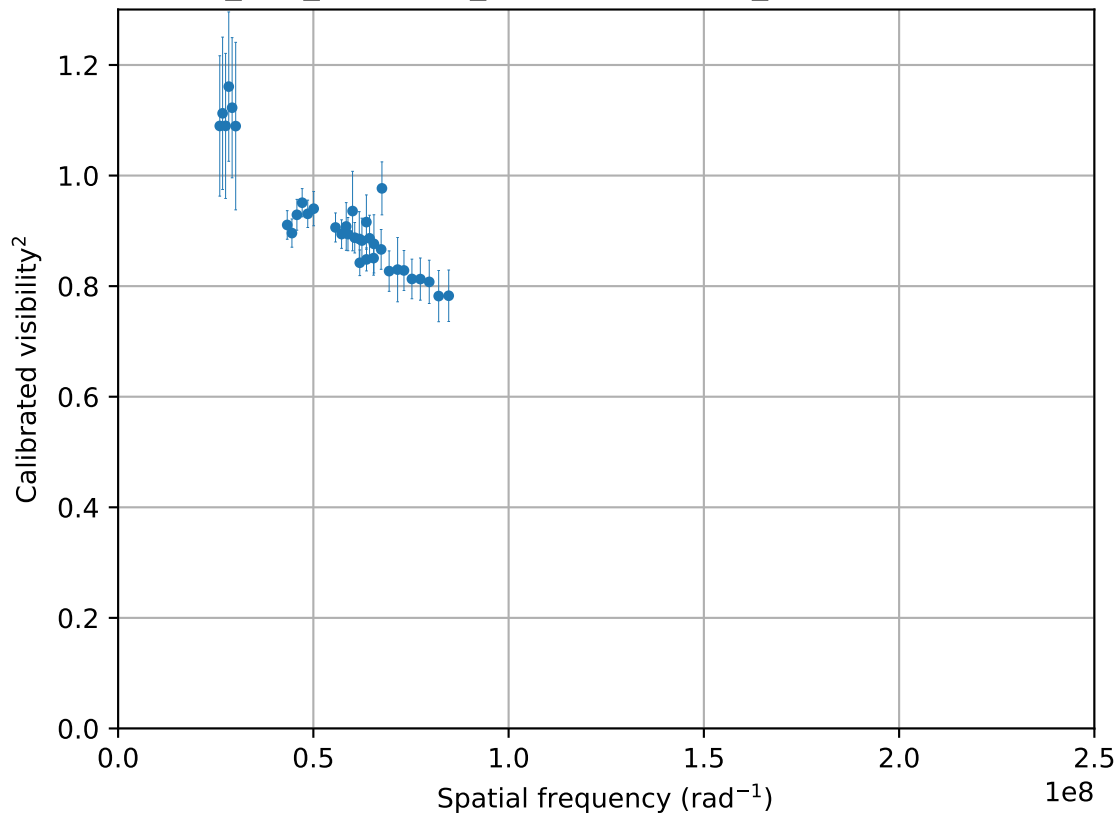
2021-02-17_CAL_HD65181_oidataCalibrated_499 (36 valid vis 2 points)
