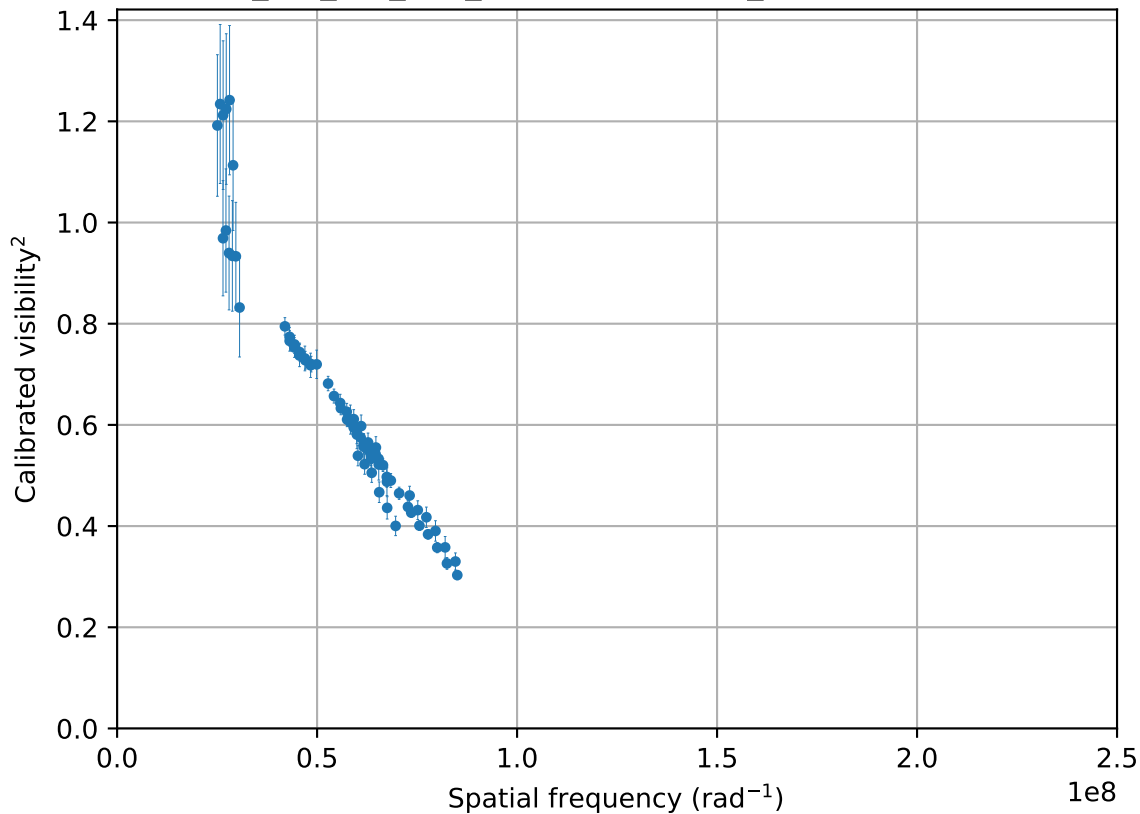
2021-02-17_SCI_rho_Pup_oidataCalibrated_499 (72 valid vis 2 points)
