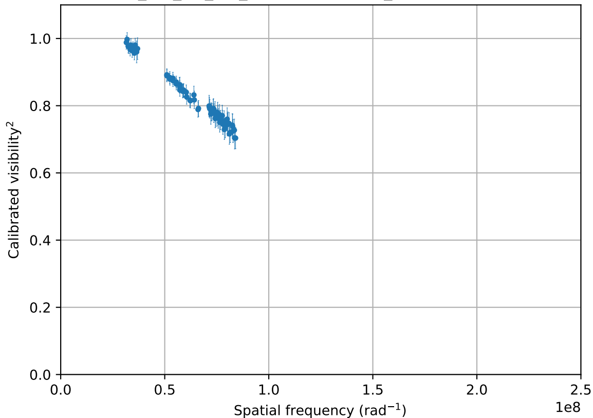
2021-03-05_SCI_psi_Vel_oidataCalibrated_499 (72 valid vis 2 points)
