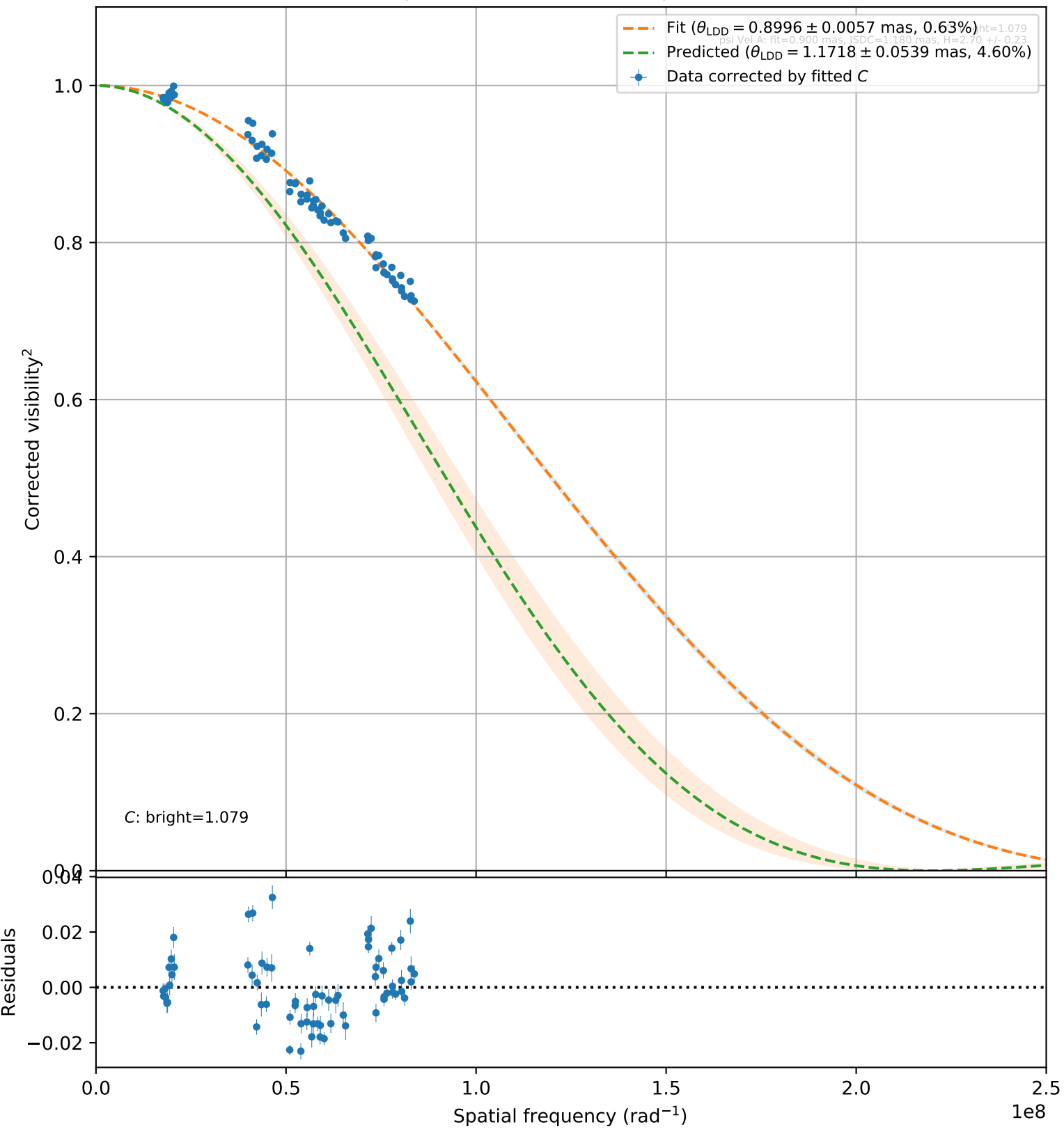
psi Vel A (72 valid vis 2 points)
