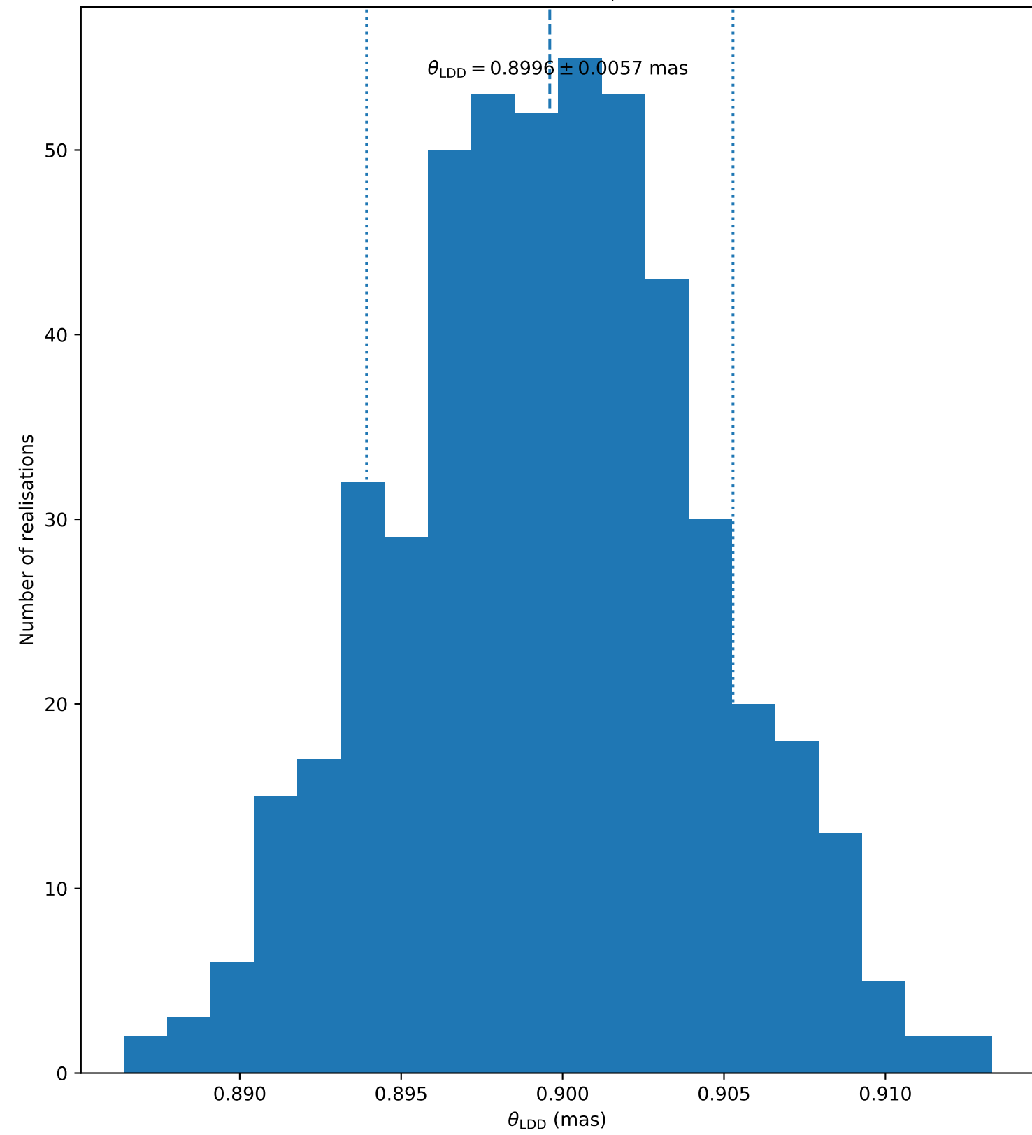
psi Vel A ( N_{\text{bootstrap}} = 500 )
