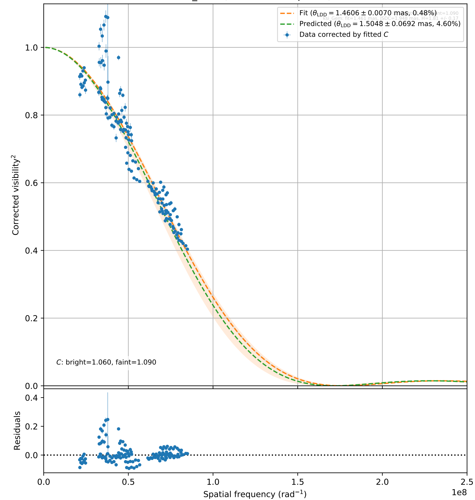
ksi_Gem (144 valid vis 2 points)
