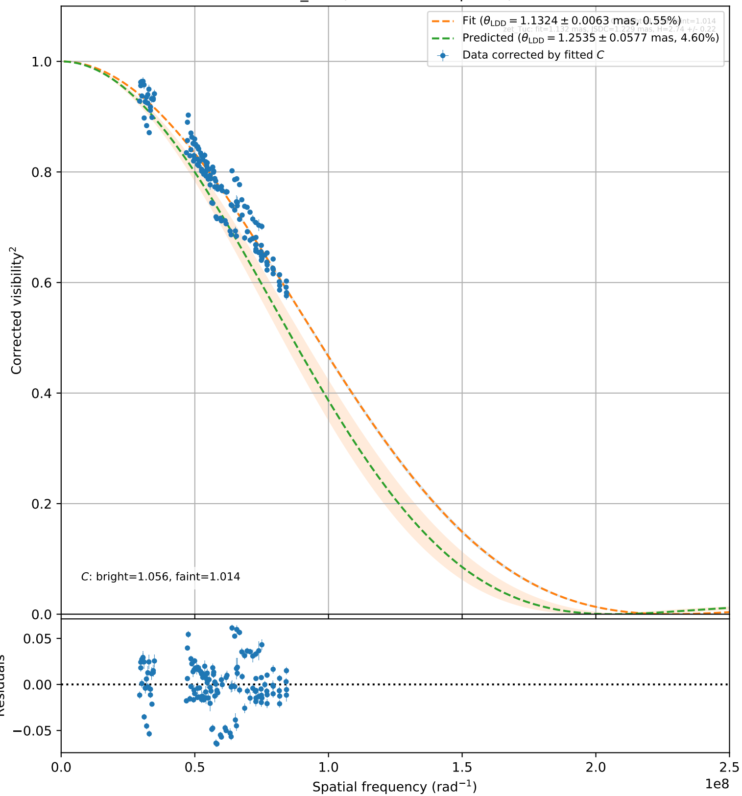
zet_Tuc (144 valid vis 2 points)
