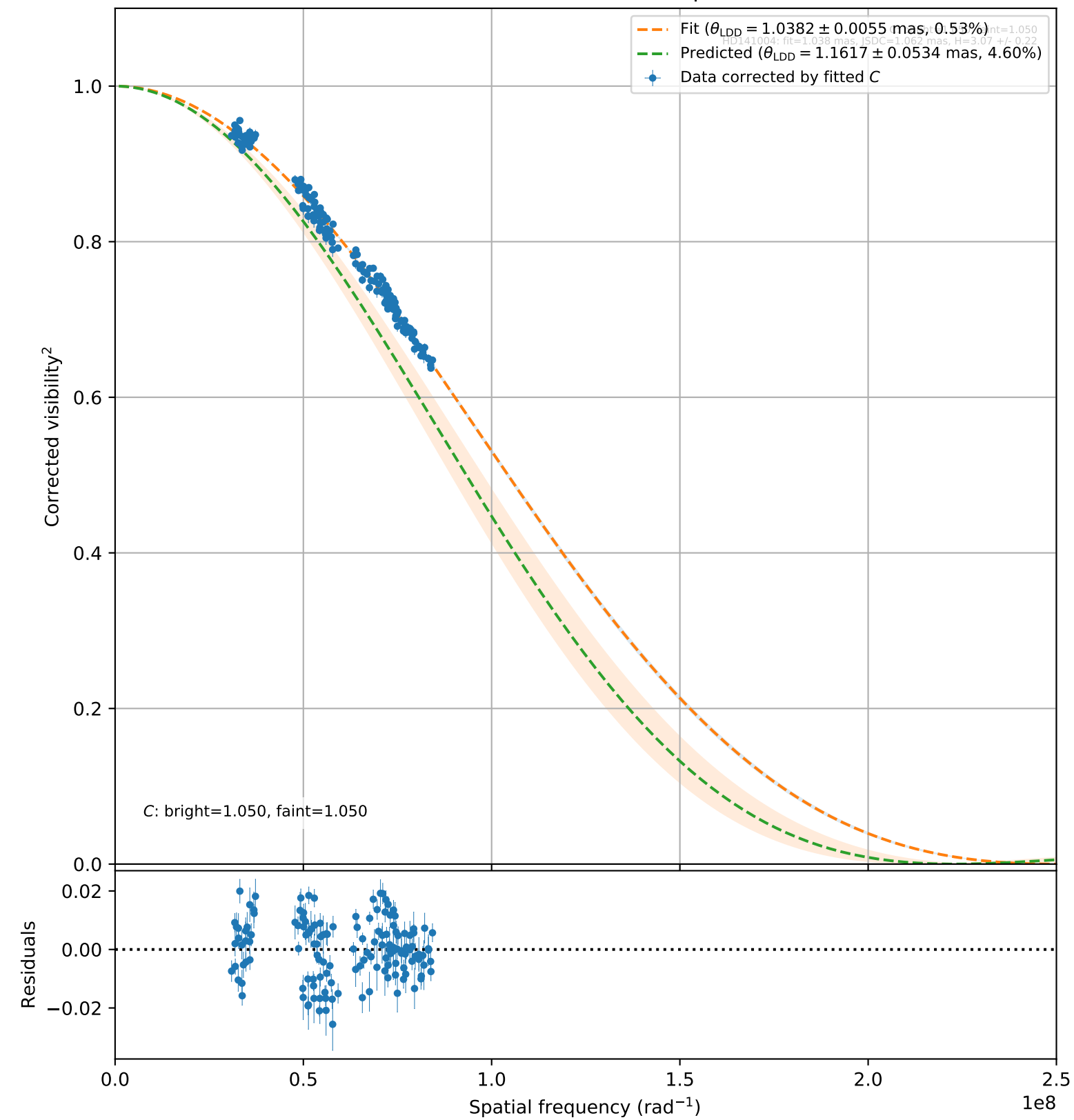
HD141004 (144 valid vis 2 points)
