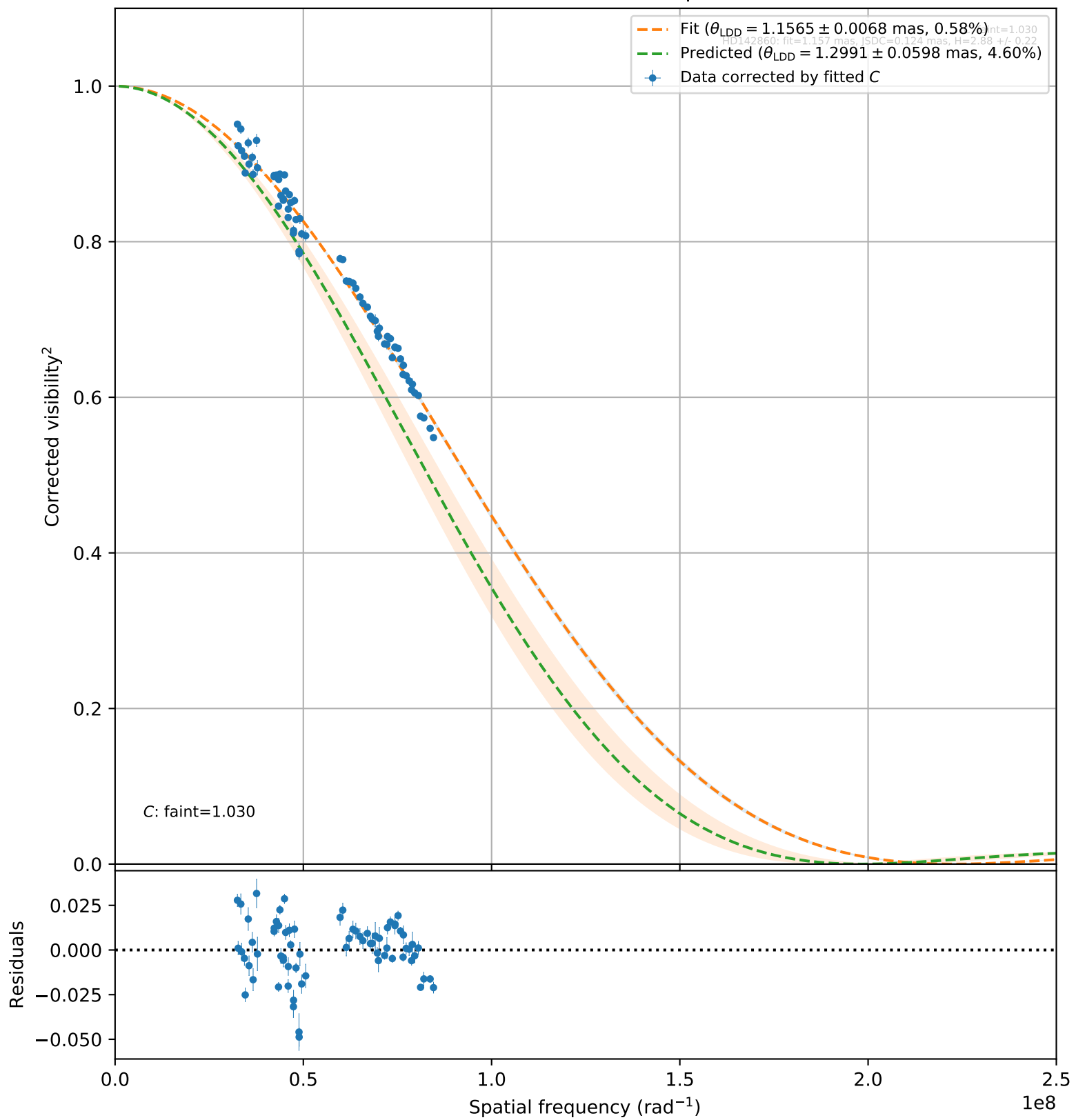
HD142860 (72 valid vis 2 points)
