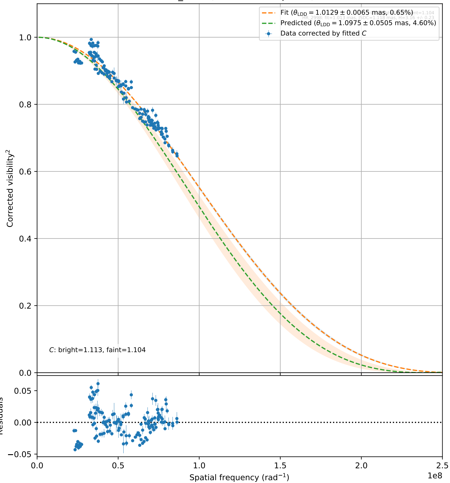
HR_2998 (144 valid vis 2 points)
