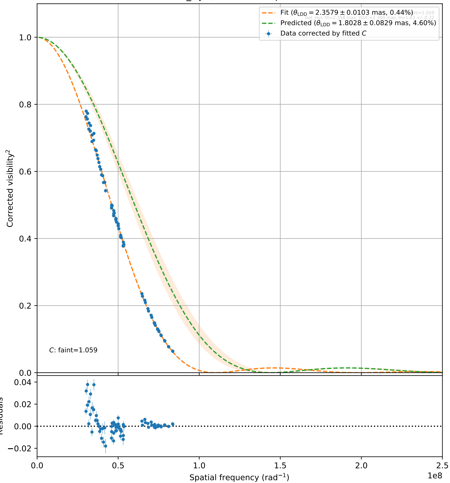
bet_Hyi (72 valid vis 2 points)
