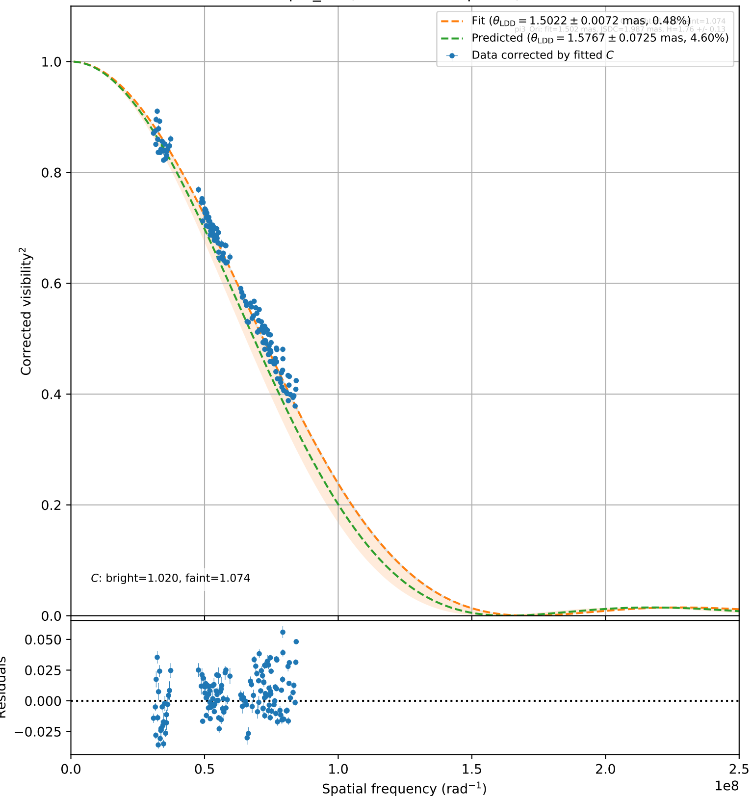
pi3_Ori (144 valid vis 2 points)
