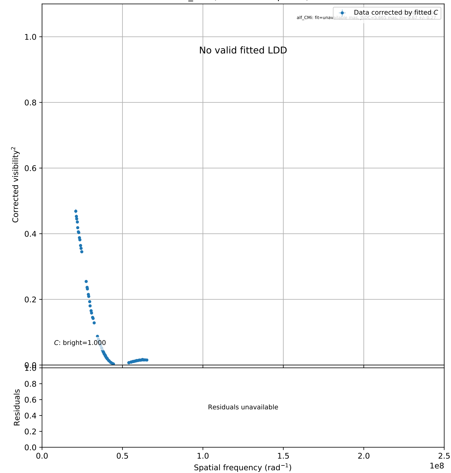
alf_CMi (72 valid vis 2 points)
