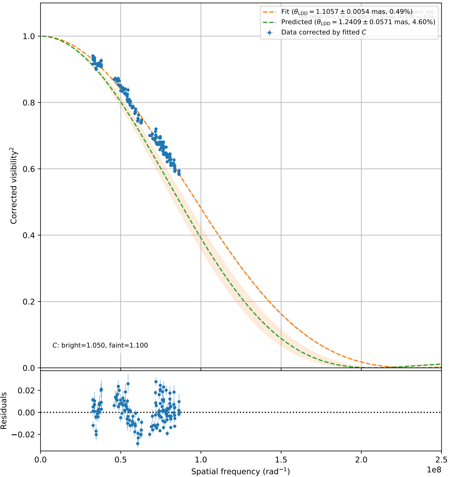
HD124850 (144 valid \text{vis}^2 points)
