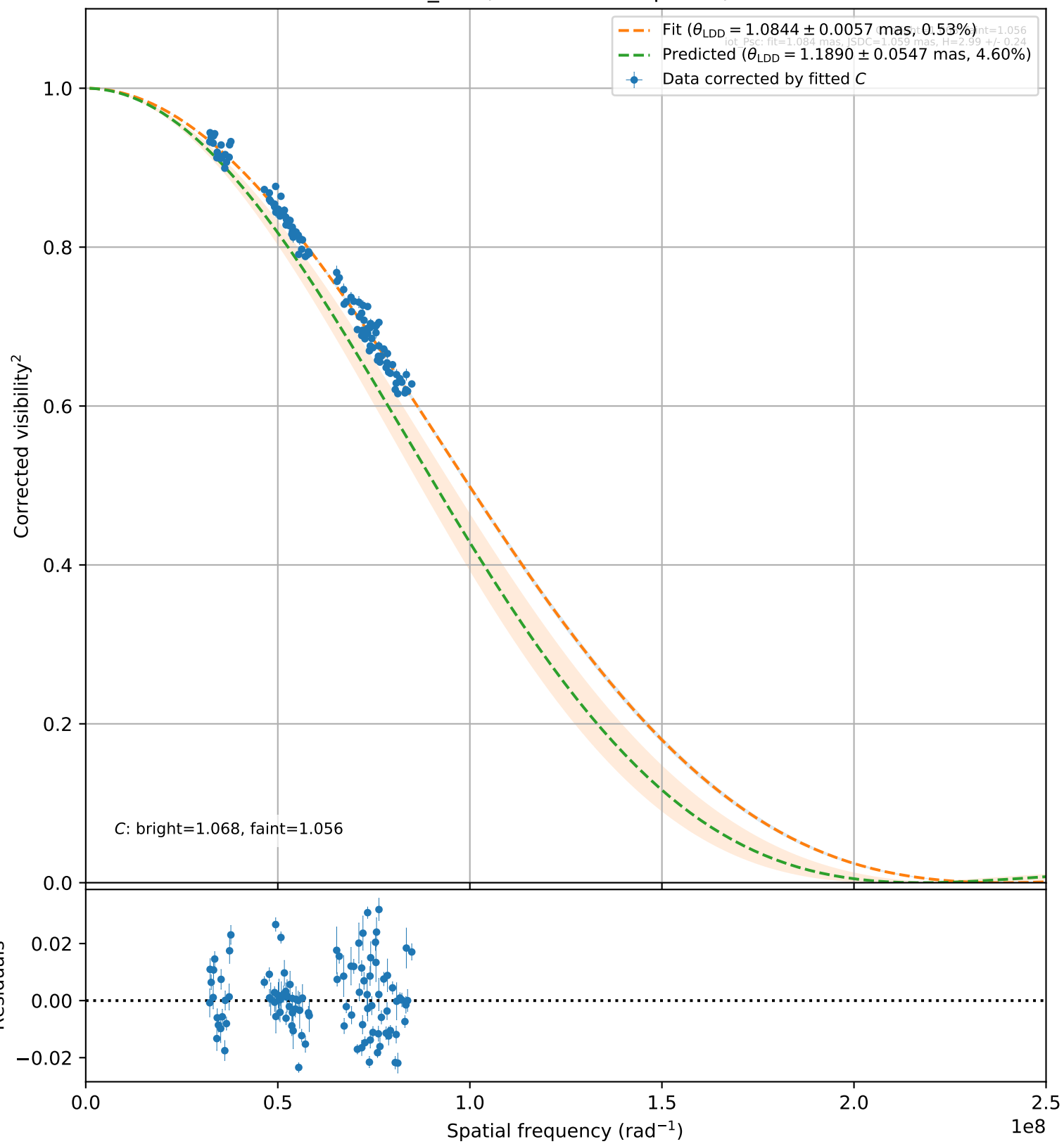
iot_Psc (108 valid vis 2 points)
