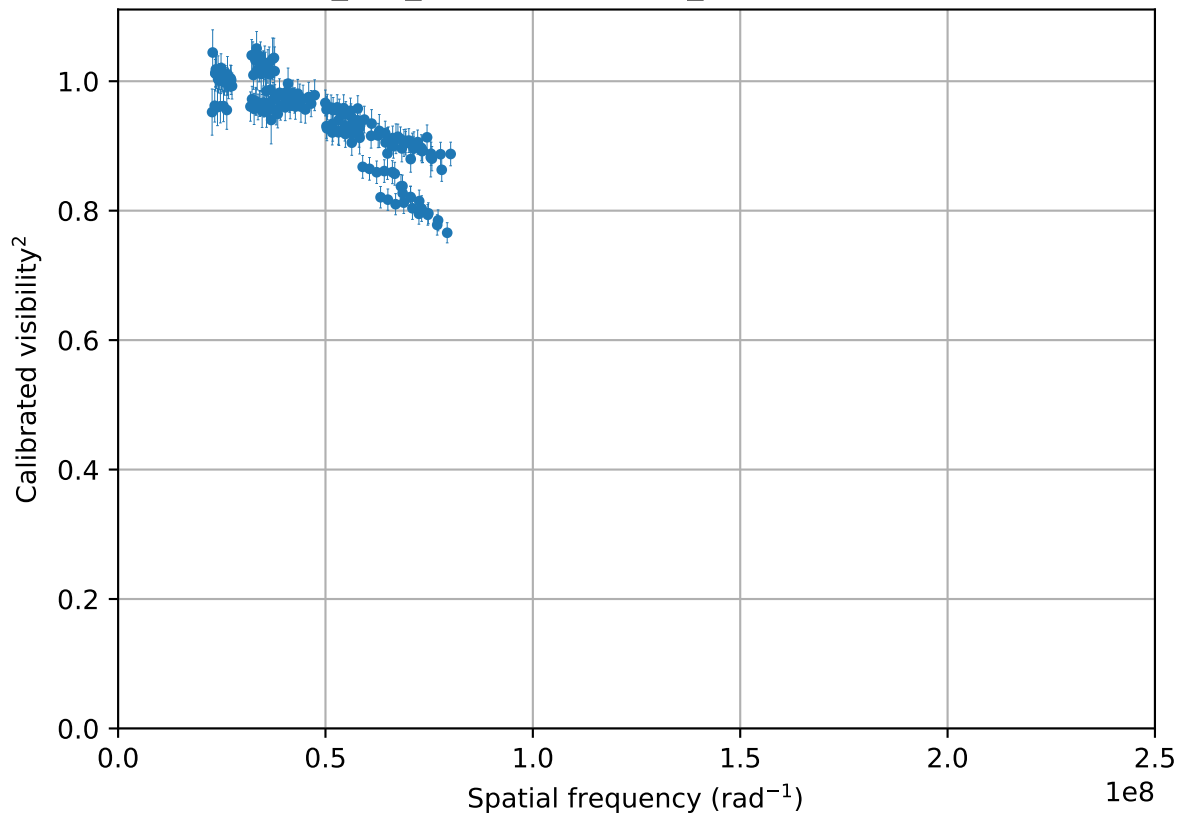
2019-11-25_ALL_oidataCalibrated_999 (180 valid vis 2 points)
