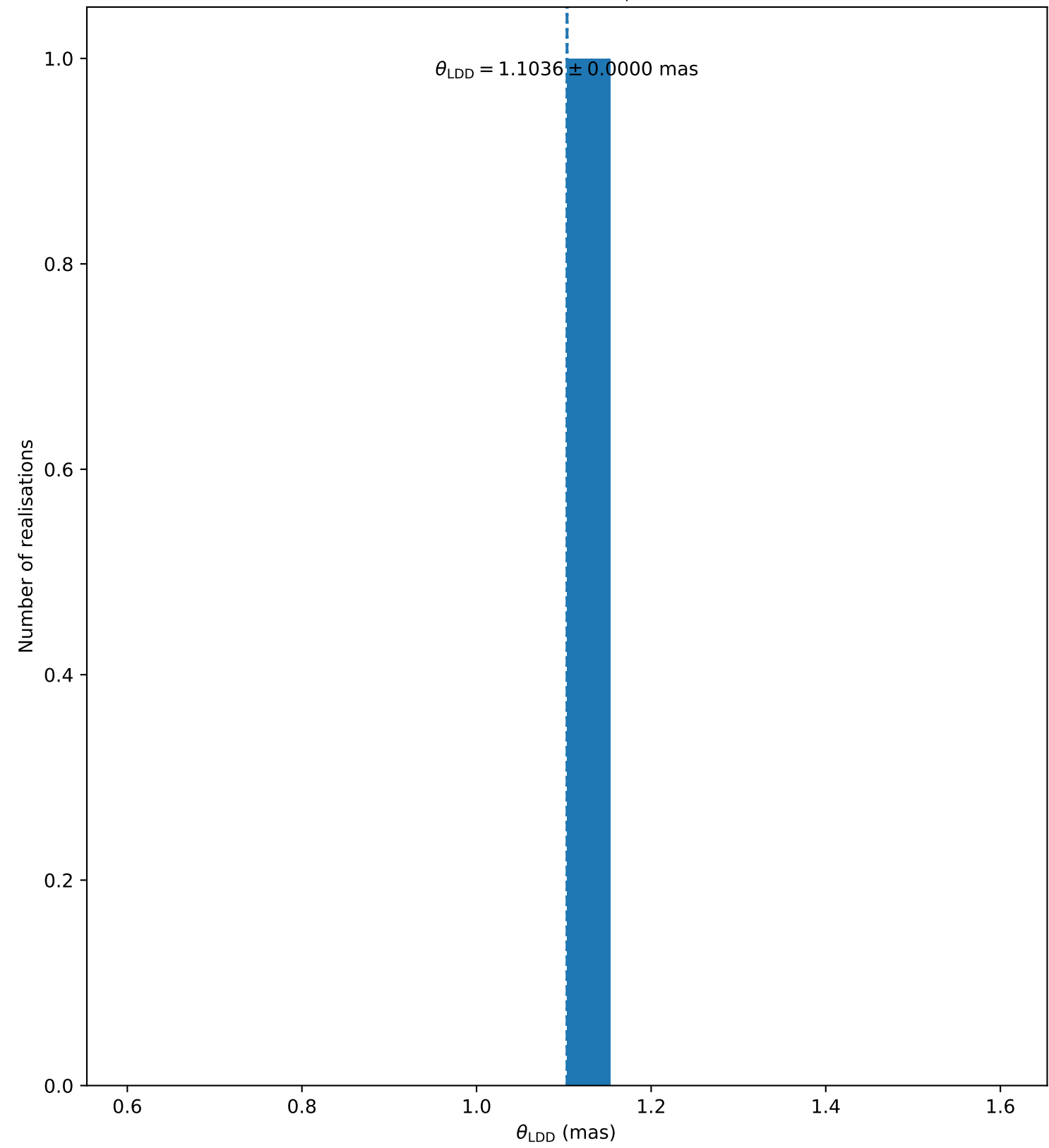
iot_Psc ( N_{\text{bootstrap}} = 1 )
