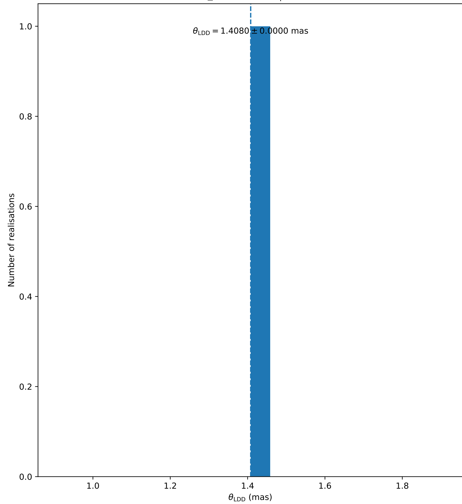
ksi_Gem ( N_{\text{bootstrap}} = 1 )
