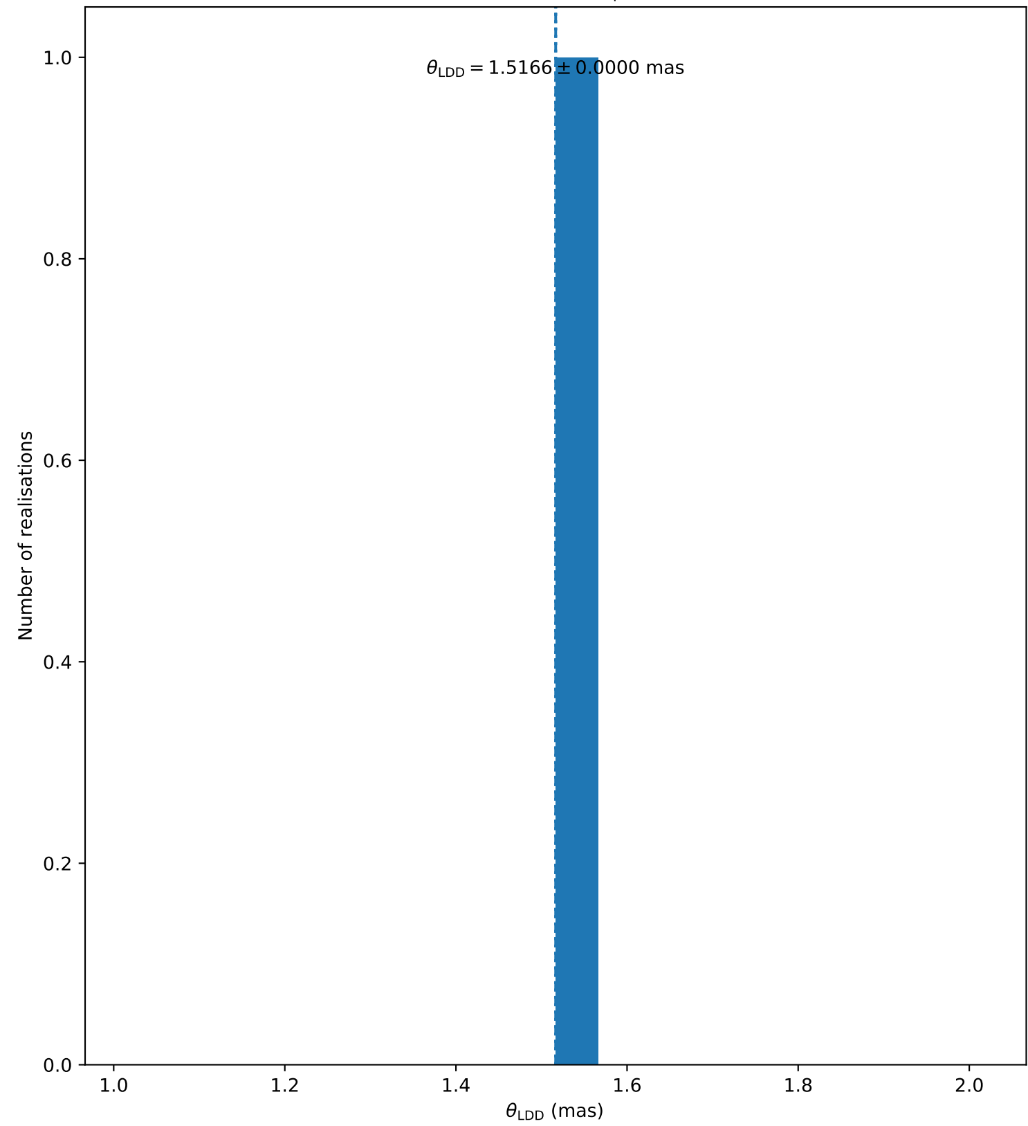
pi3_Ori ( N_{\text{bootstrap}} = 1 )
