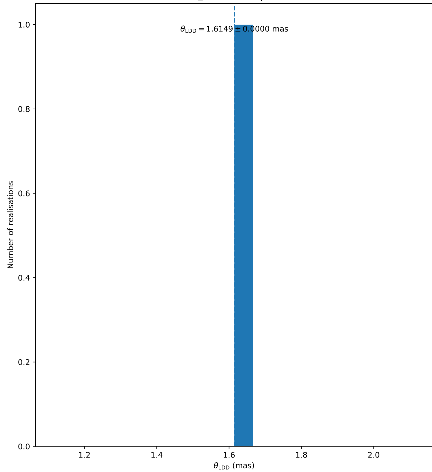
rho_Pup ( N_{\text{bootstrap}} = 1 )
