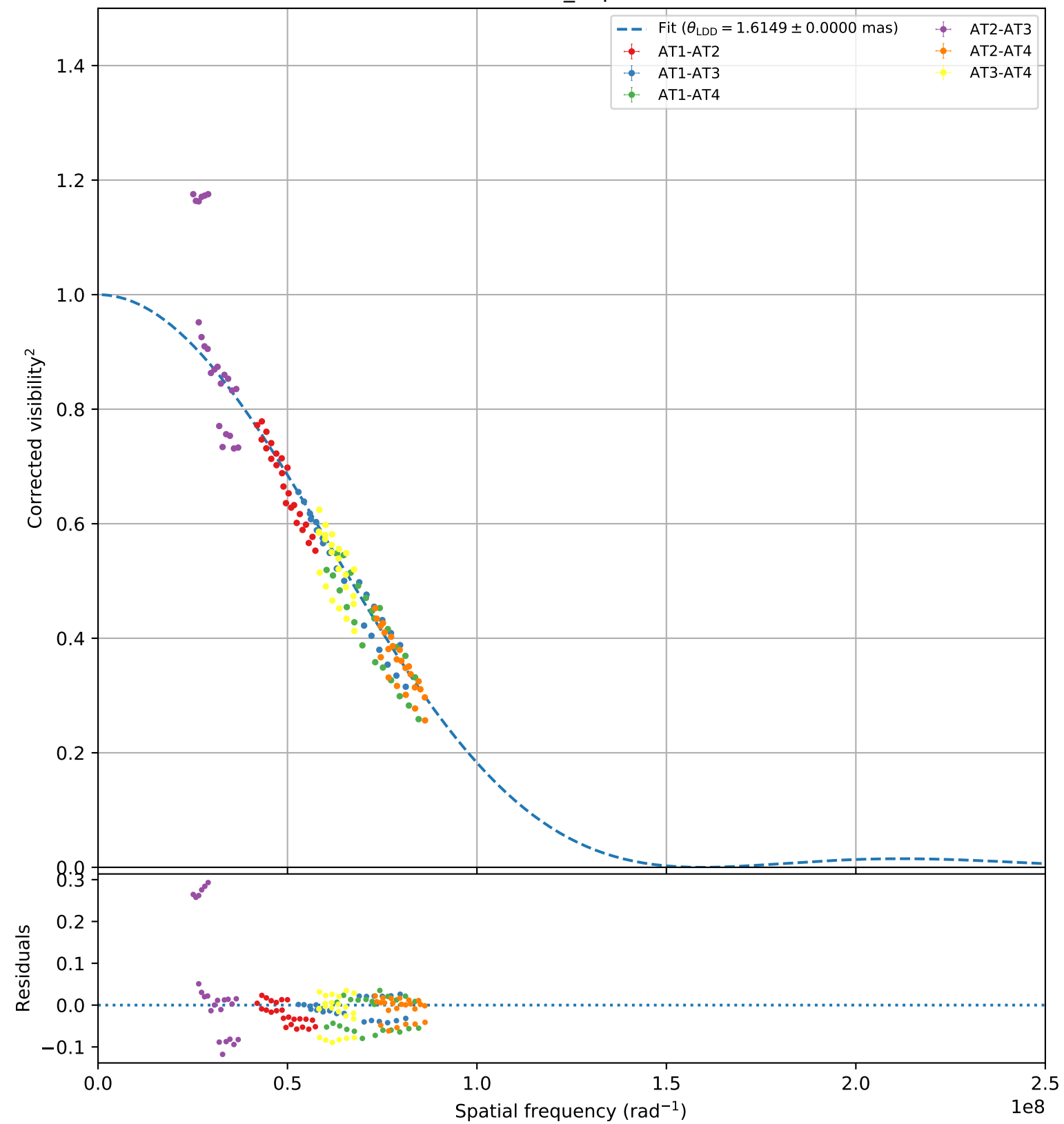
rho_Pup
