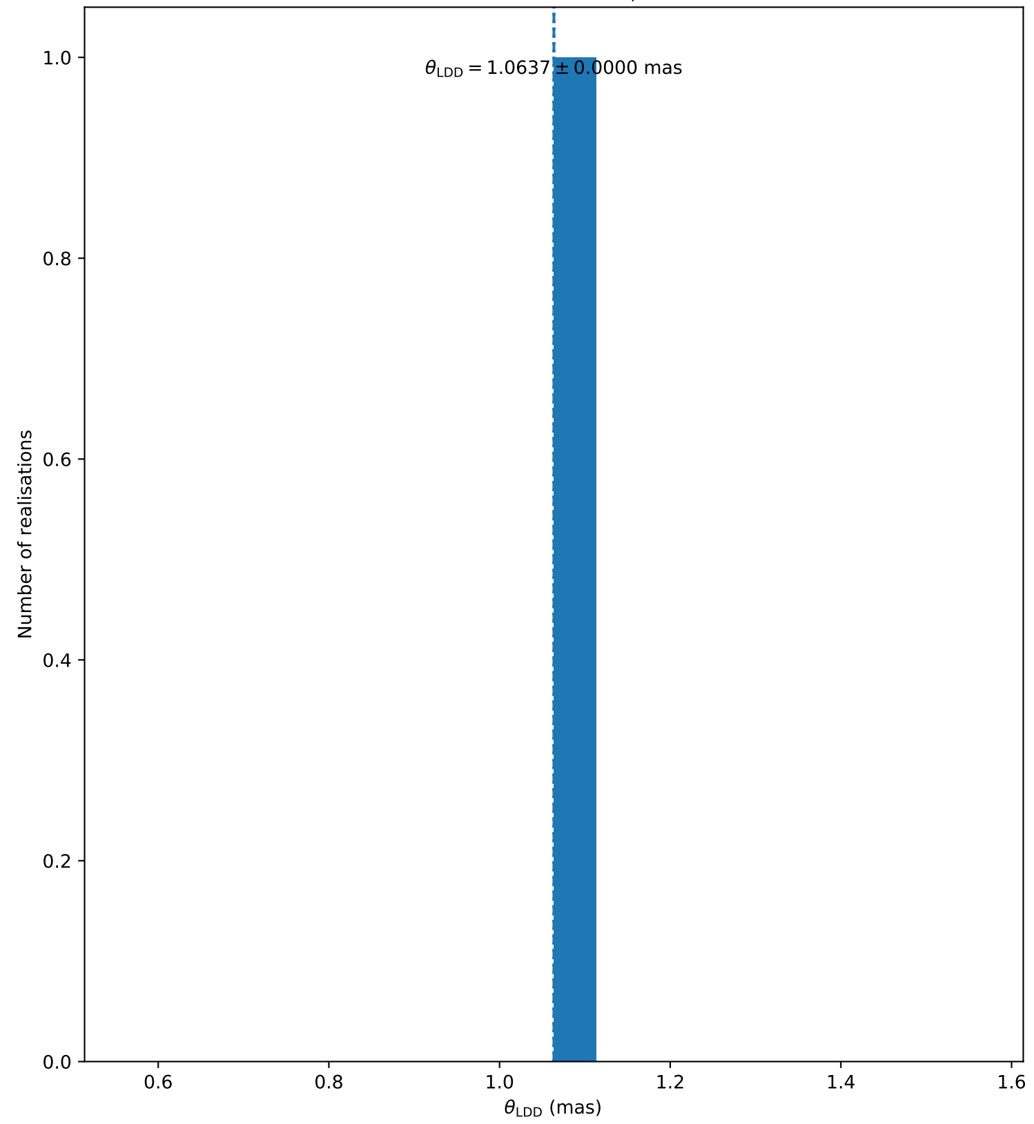
HD141004 ( N_{\text{bootstrap}} = 1 )
