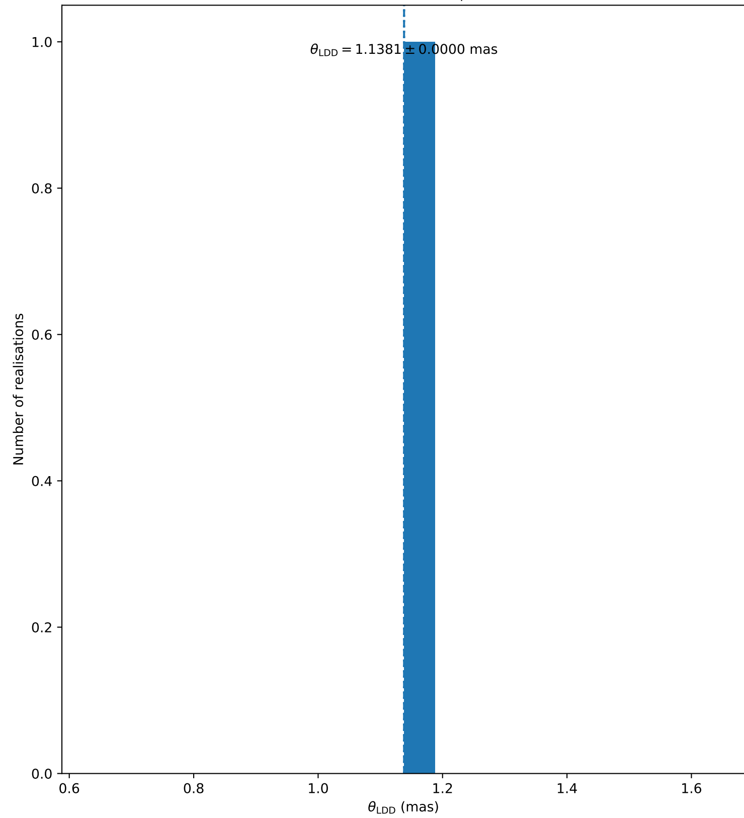
HD124850 ( N_{\text{bootstrap}} = 1 )
