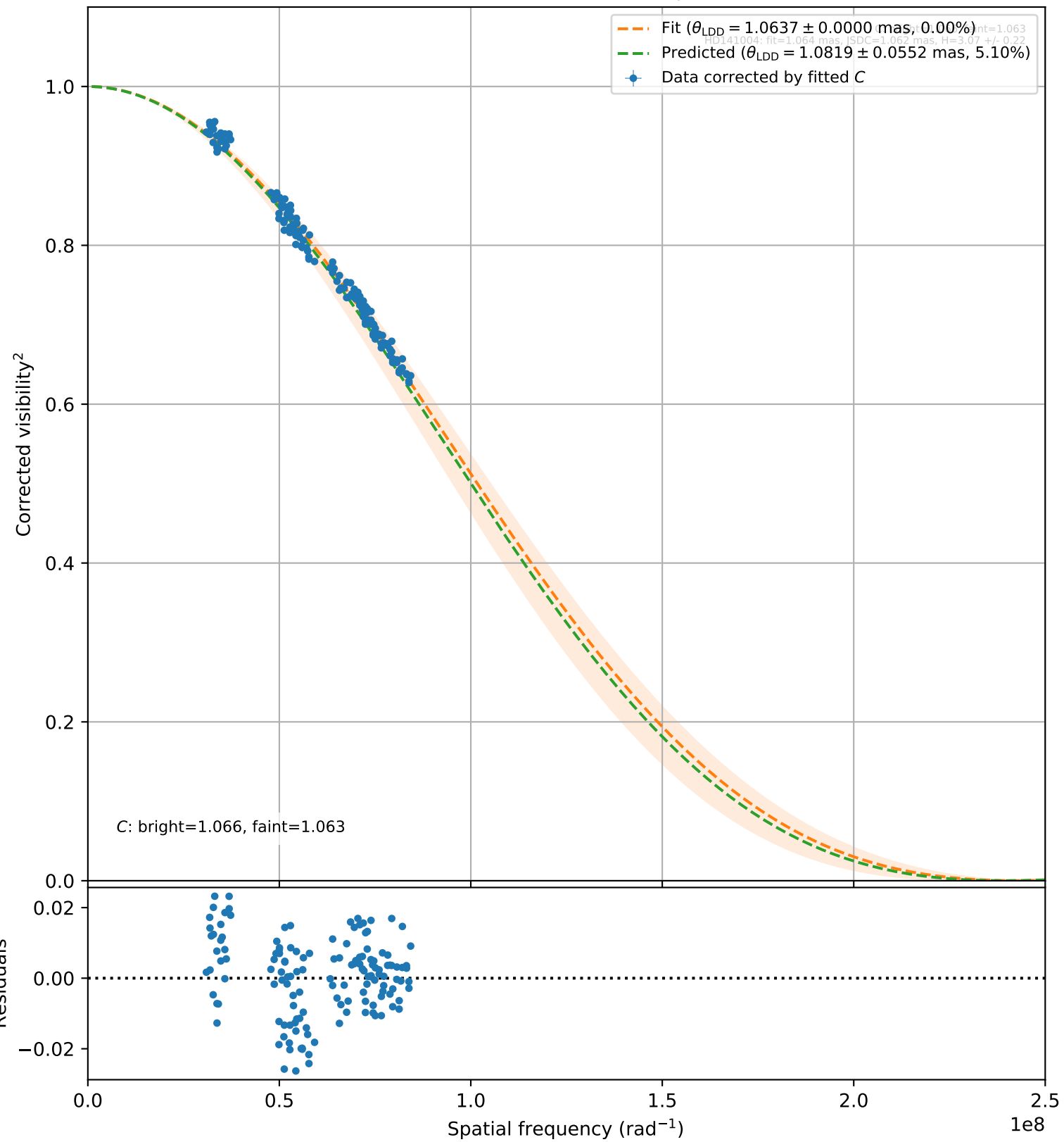
HD141004 (144 valid vis 2 points)
