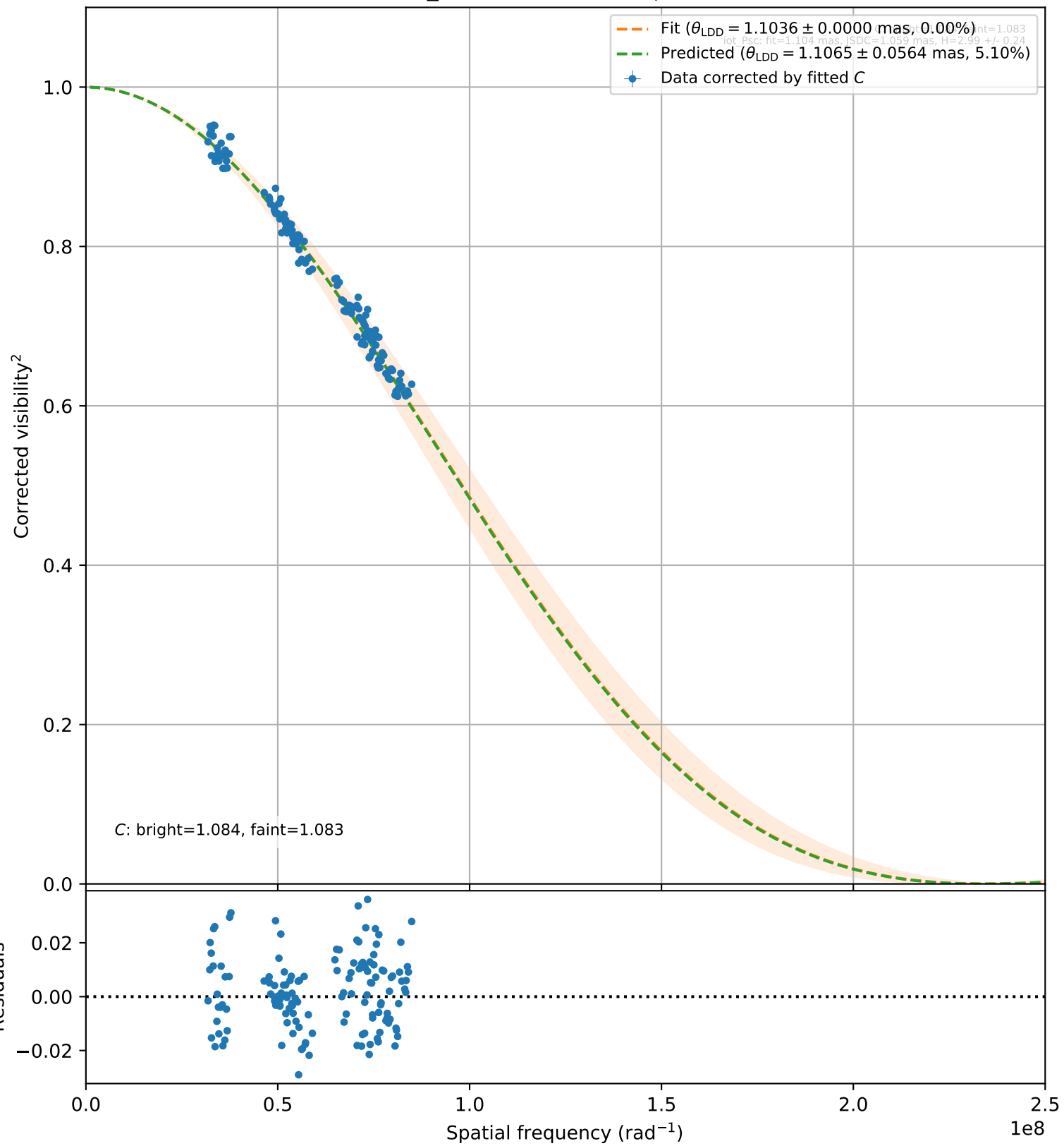
iot_Psc (144 valid vis 2 points)
