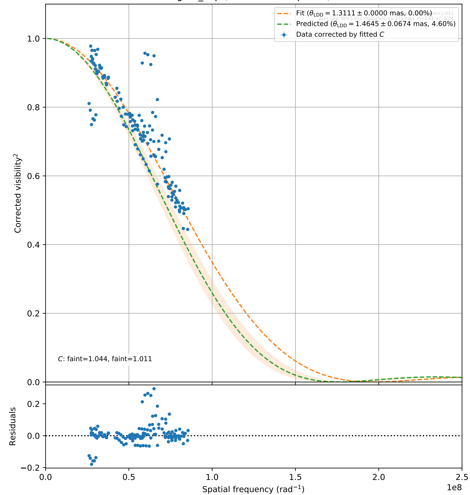
gam_Lep (144 valid vis 2 points)
