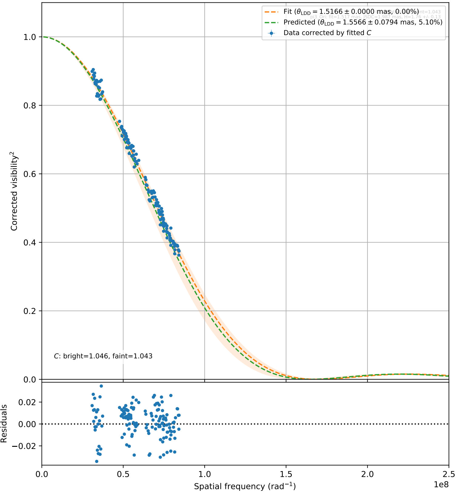
pi3_Ori (144 valid vis 2 points)
