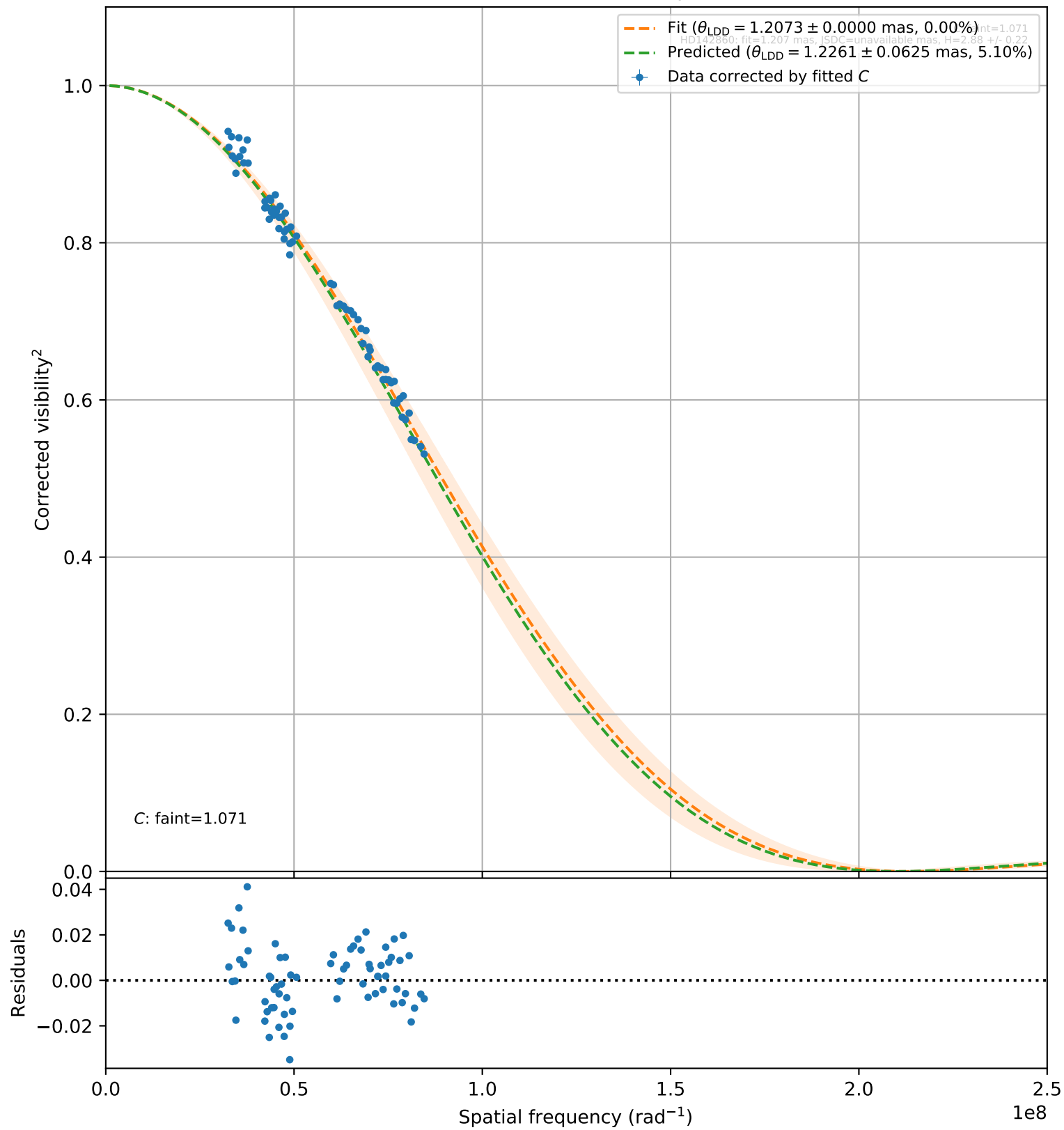
HD142860 (72 valid \text{vis}^2 points)
