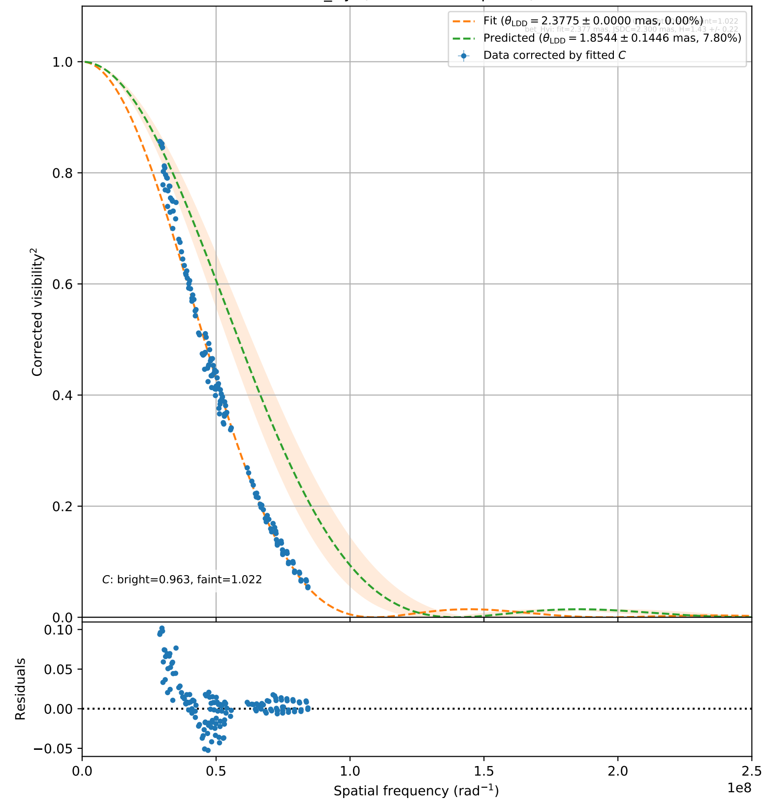
bet_Hyi (144 valid vis 2 points)
