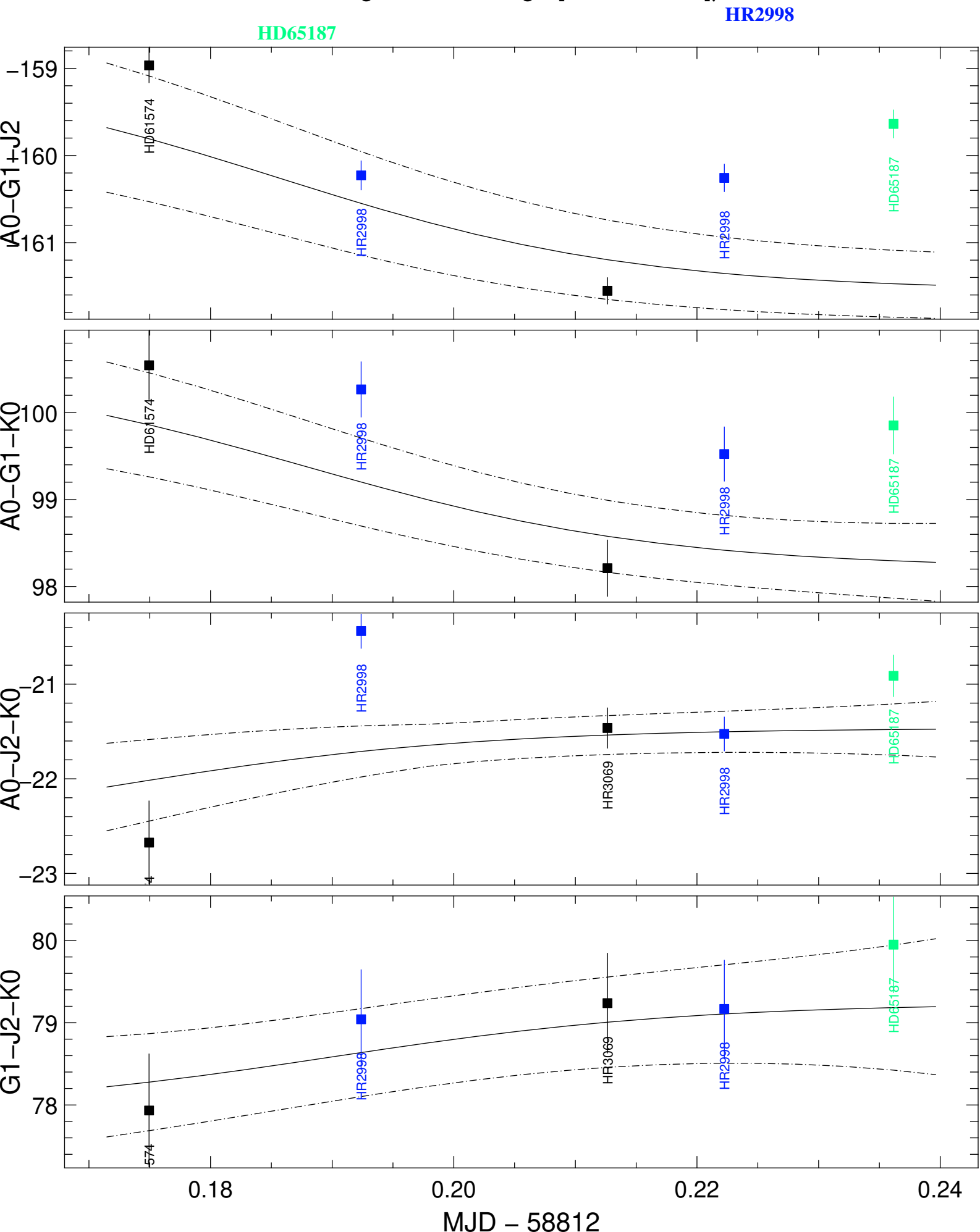
Transfer-Function t3Phi (black) and Scientific t3Phi (colors) averaged in the range [1.677, 1.677] \mu\text{m}
