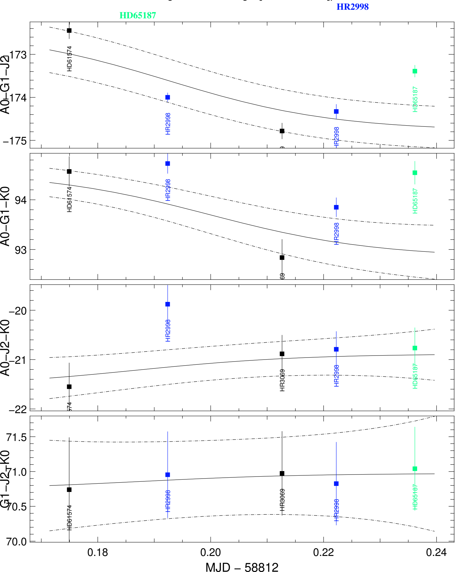
Transfer-Function t3Phi (black) and Scientific t3Phi (colors) averaged in the range [1.773,1.773] \mu m
