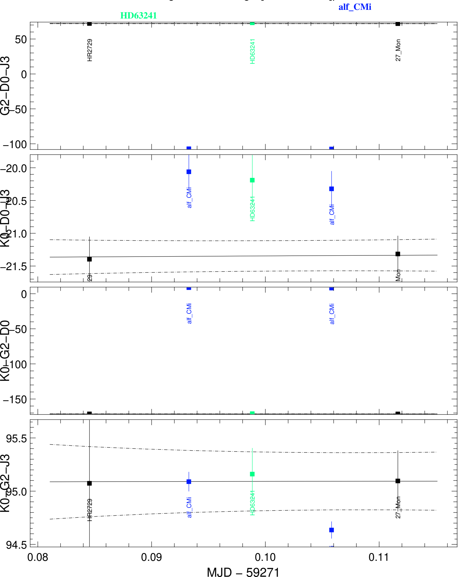
Transfer-Function t3Phi (black) and Scientific t3Phi (colors) averaged in the range [1.725, 1.725] \mu\text{m}
