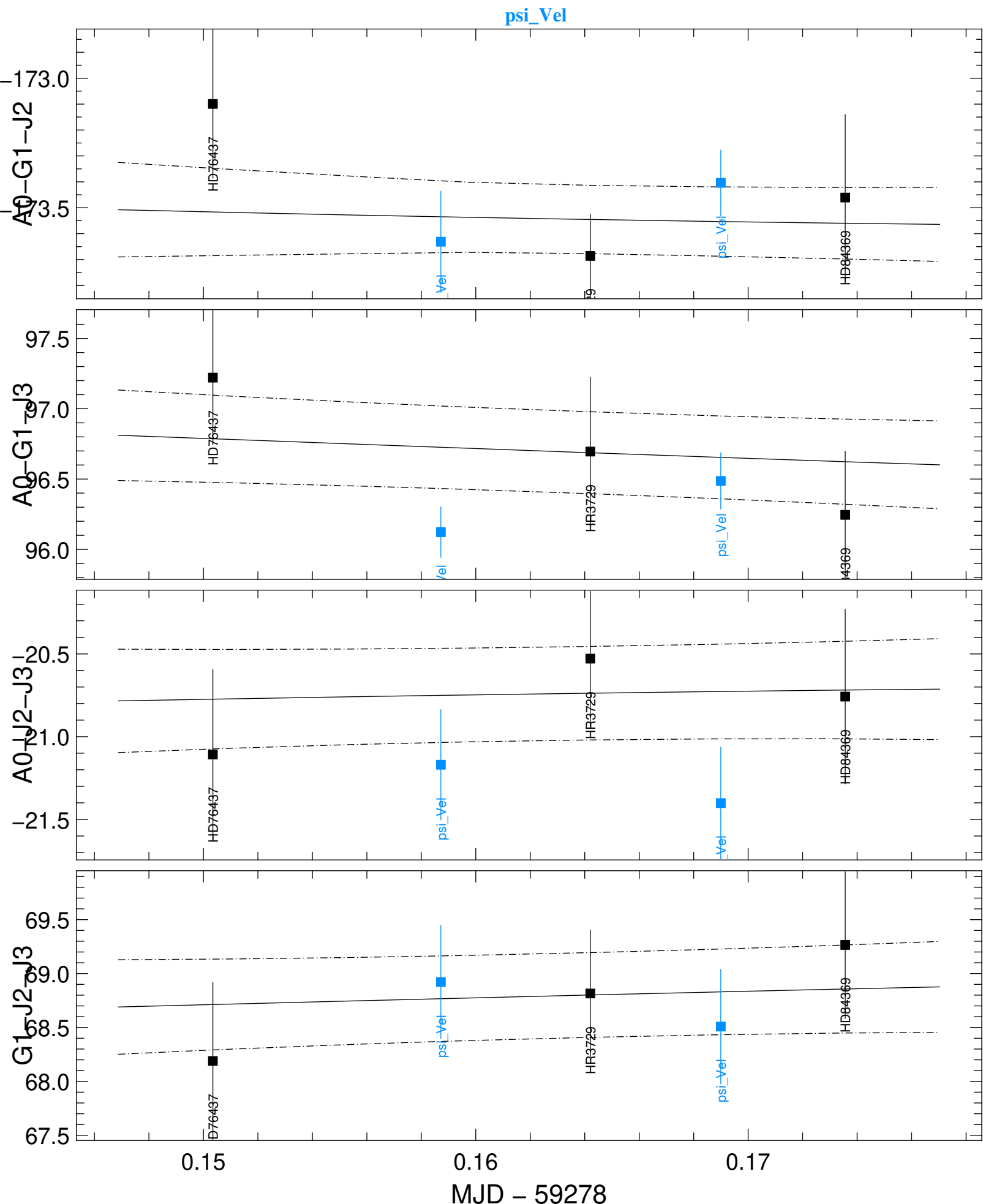
Transfer-Function t3Phi (black) and Scientific t3Phi (colors) averaged in the range [1.773,1.773] \mu\text{m}
