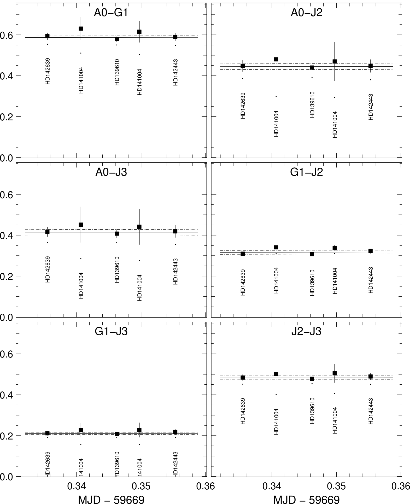
Transfer-Function vis2 (black) and Scientific vis2 (colors) averaged in the range [1.533, 1.533] \mu\text{m}
