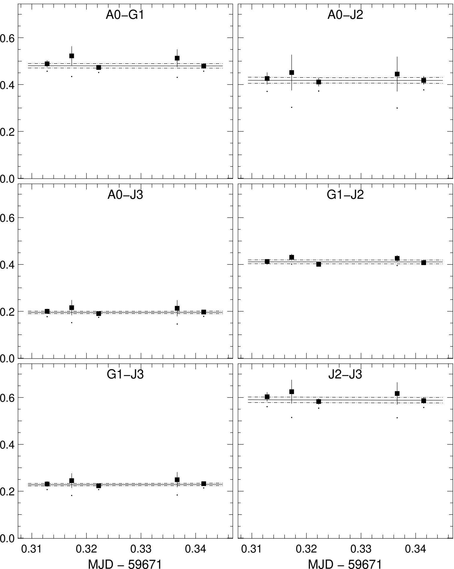
Transfer-Function vis2 (black) and Scientific vis2 (colors) averaged in the range [[1.637, 1.715], [2.04, 2.25]] \mu\text{m}
