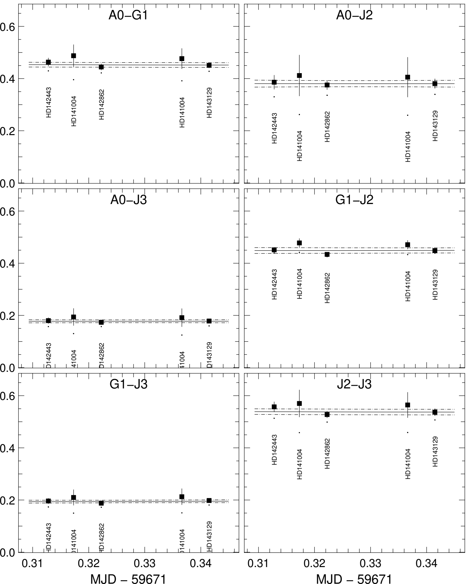
Transfer-Function vis2 (black) and Scientific vis2 (colors) averaged in the range [1.581, 1.581]\mu\text{m}
