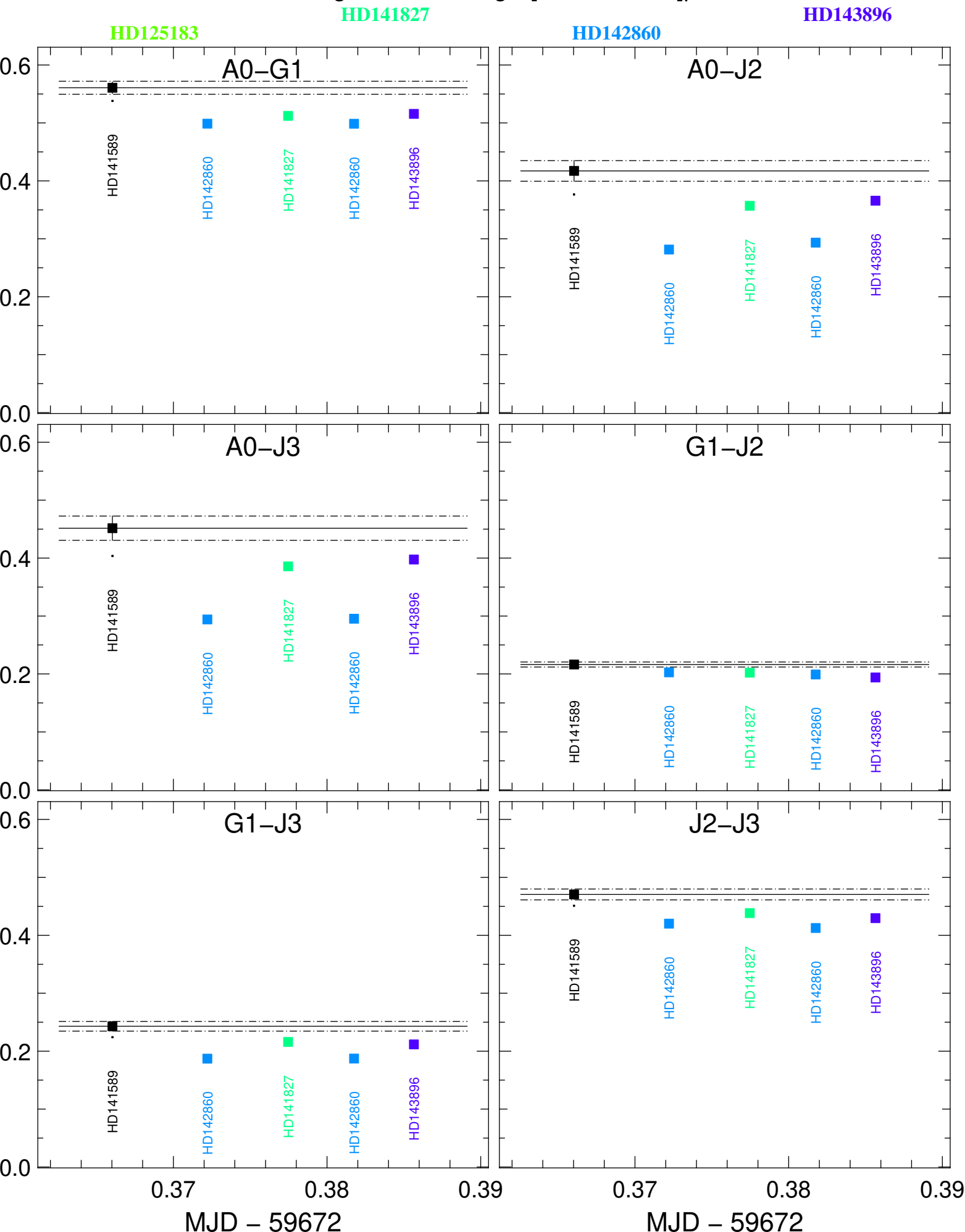
Transfer-Function vis2 (black) and Scientific vis2 (colors) averaged in the range [1.677, 1.677]\mu\text{m}
