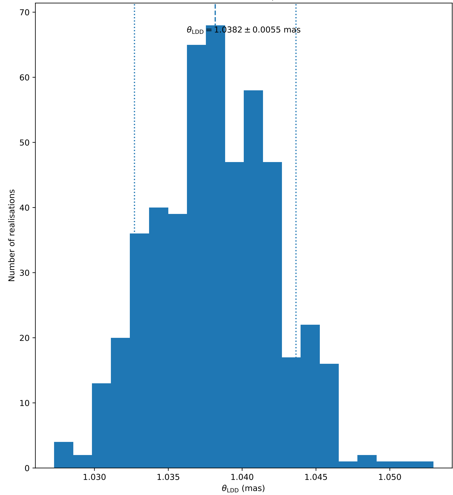
HD141004 ( N_{\text{bootstrap}} = 500 )
