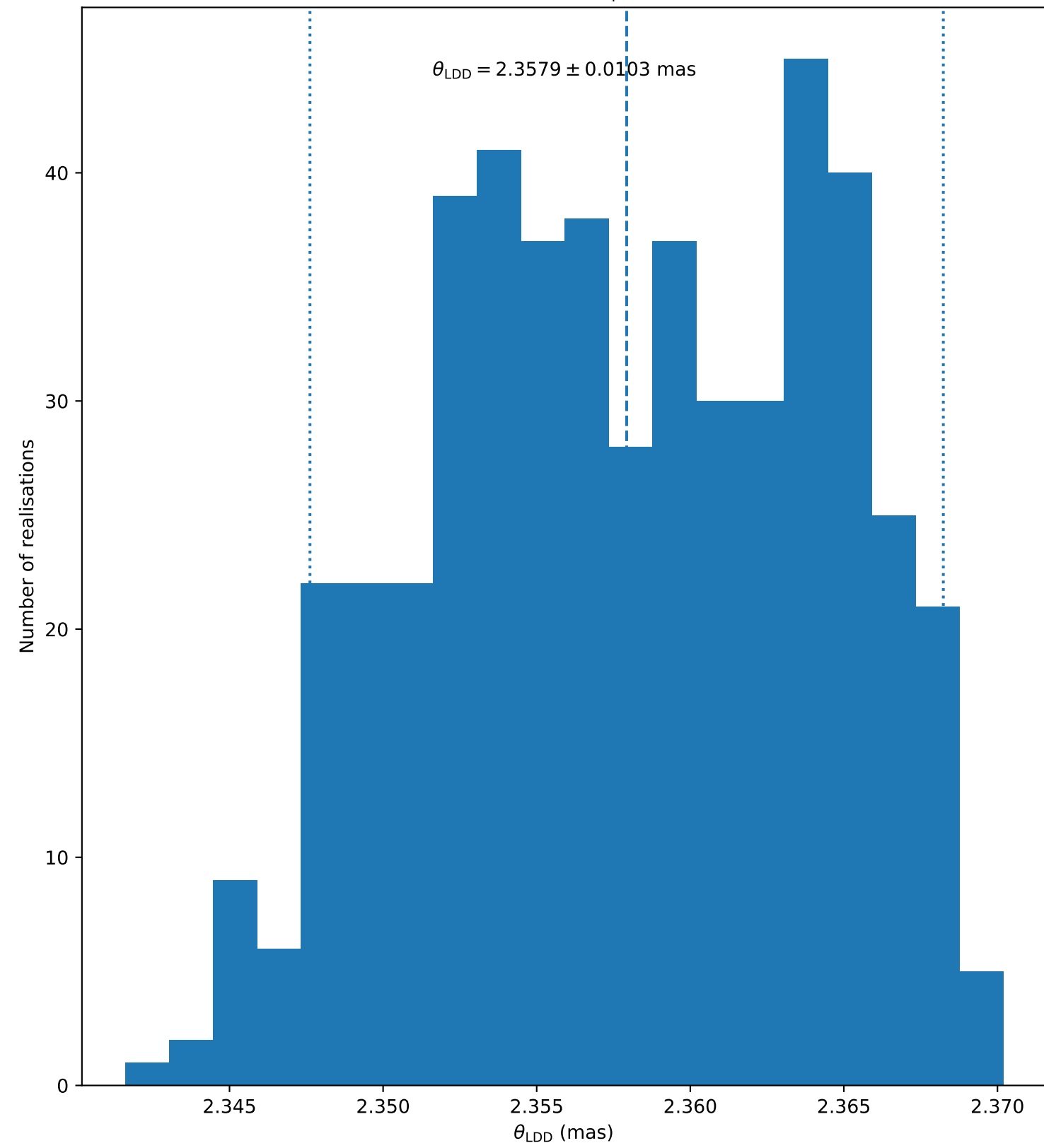
bet_Hyi ( N_{\text{bootstrap}} = 500 )
