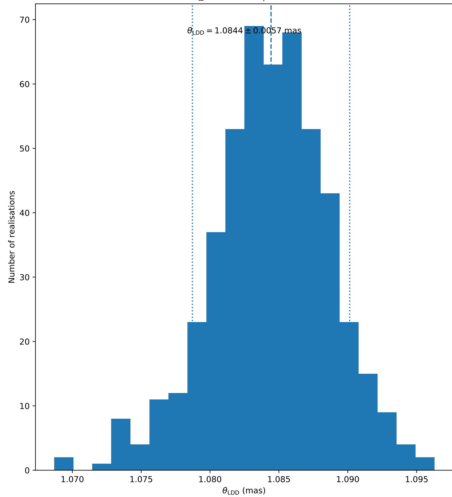
iot_Psc ( N_{\text{bootstrap}} = 500 )
