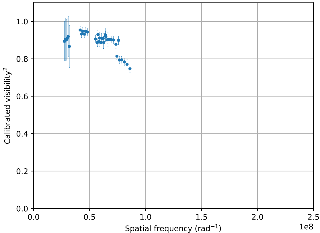
2021-02-17_CAL_HD70942_oidataCalibrated_499 (36 valid vis 2 points)
