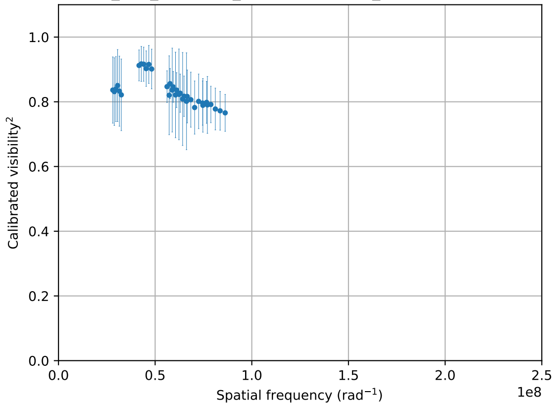
2021-02-18_CAL_HD42747_oidataCalibrated_499 (36 valid vis 2 points)
