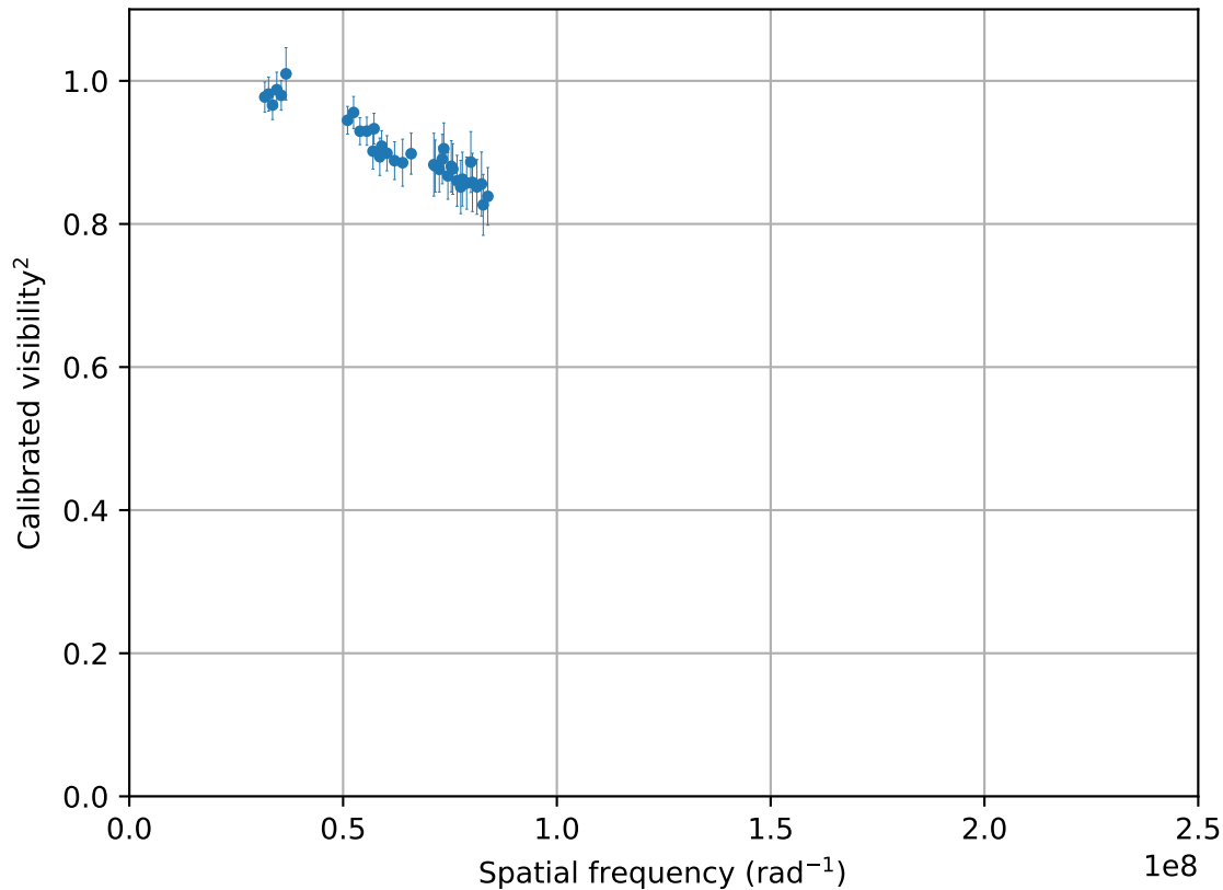
2021-03-05_CAL_HD84369_oidataCalibrated_499 (36 valid vis 2 points)
