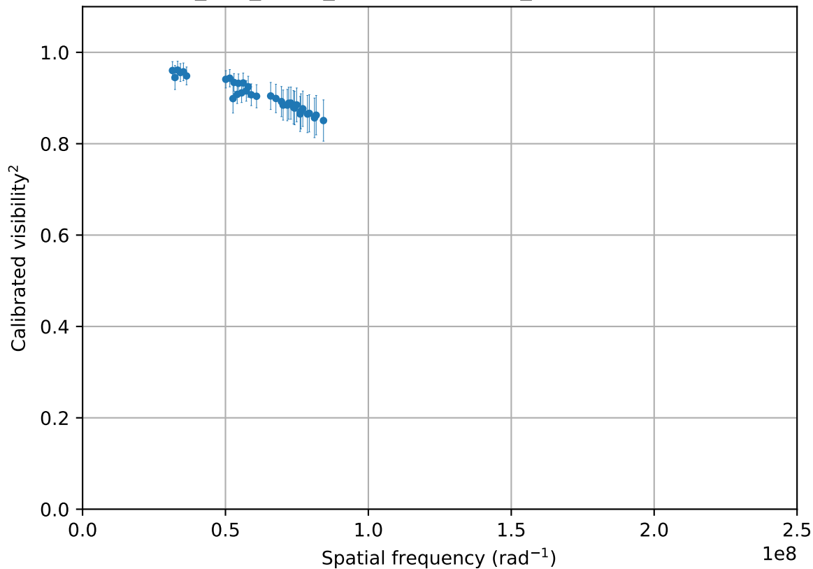
2019-11-29_CAL_HD43_oidataCalibrated_499 (36 valid vis 2 points)
