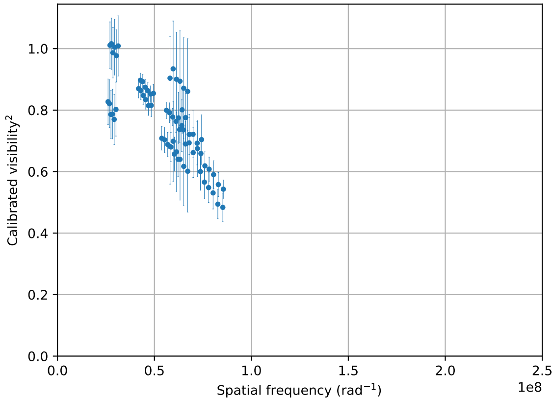
2021-02-18_SCI_gam_Lep_oidataCalibrated_499 (72 valid vis 2 points)
