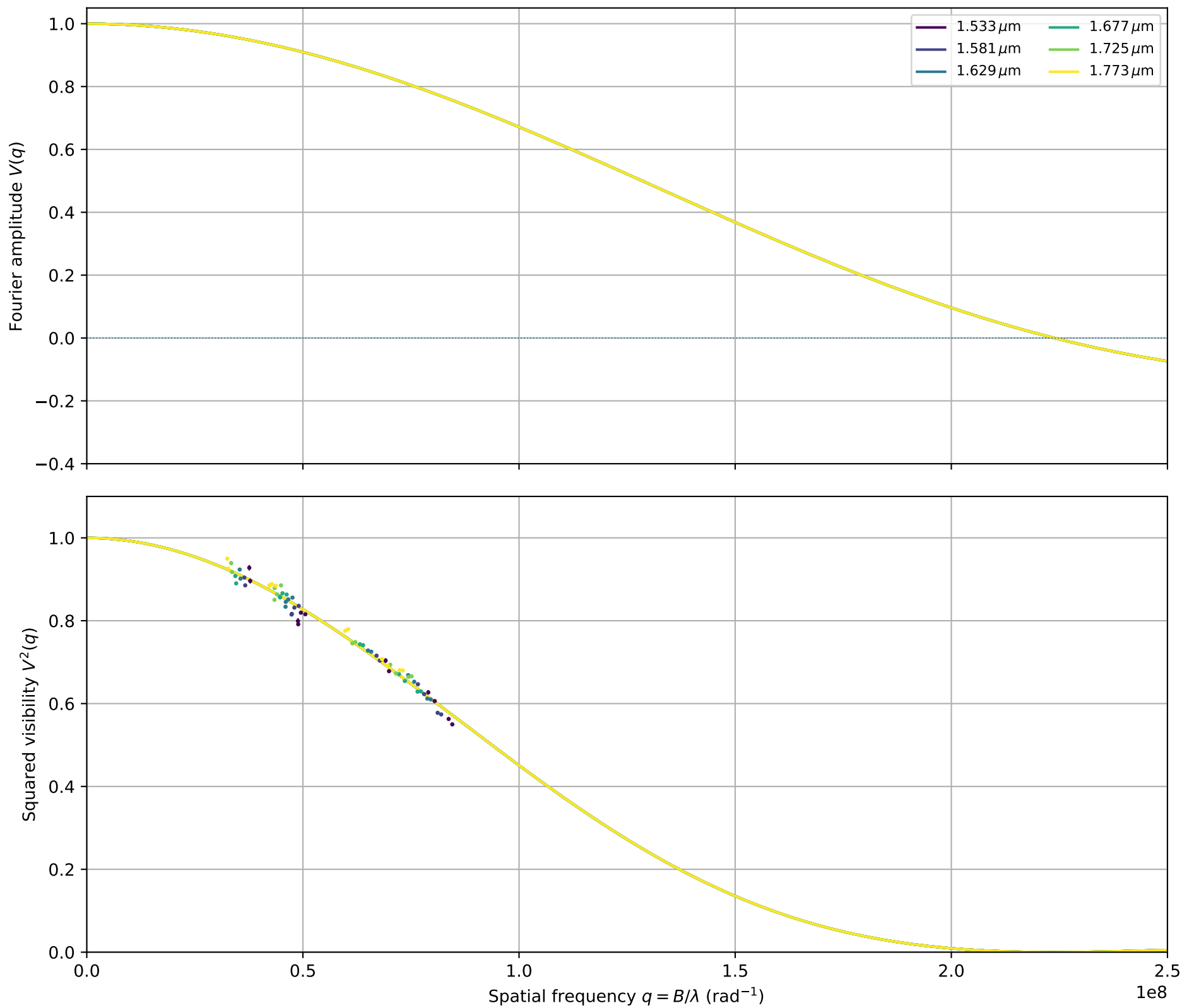
HD142860: fitted \theta_{\text{LDD}} = 1.1518 \pm 0.0045 mas
