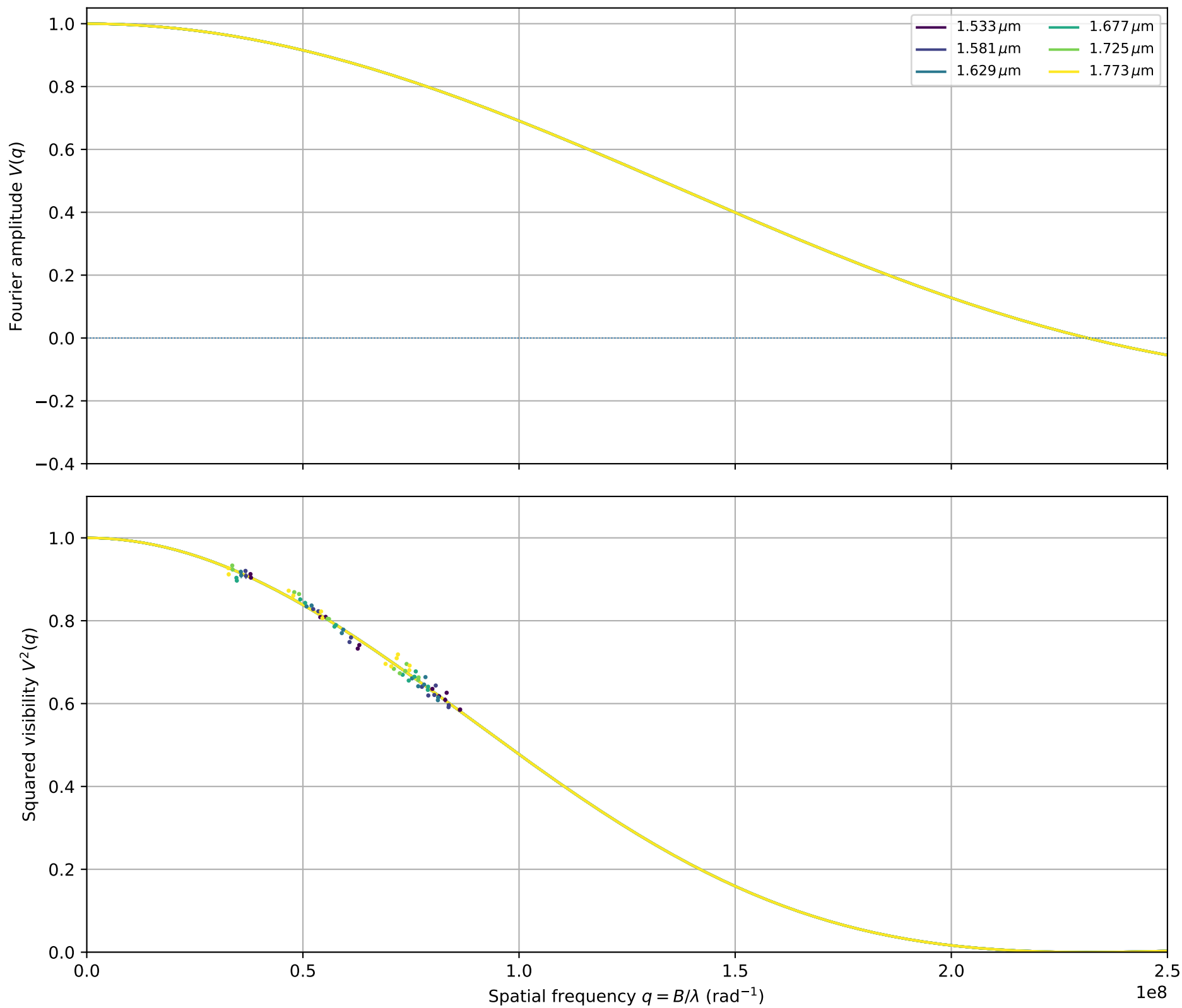
HD124850: fitted \theta_{\text{LDD}} = 1.1097 \pm 0.0038 mas
