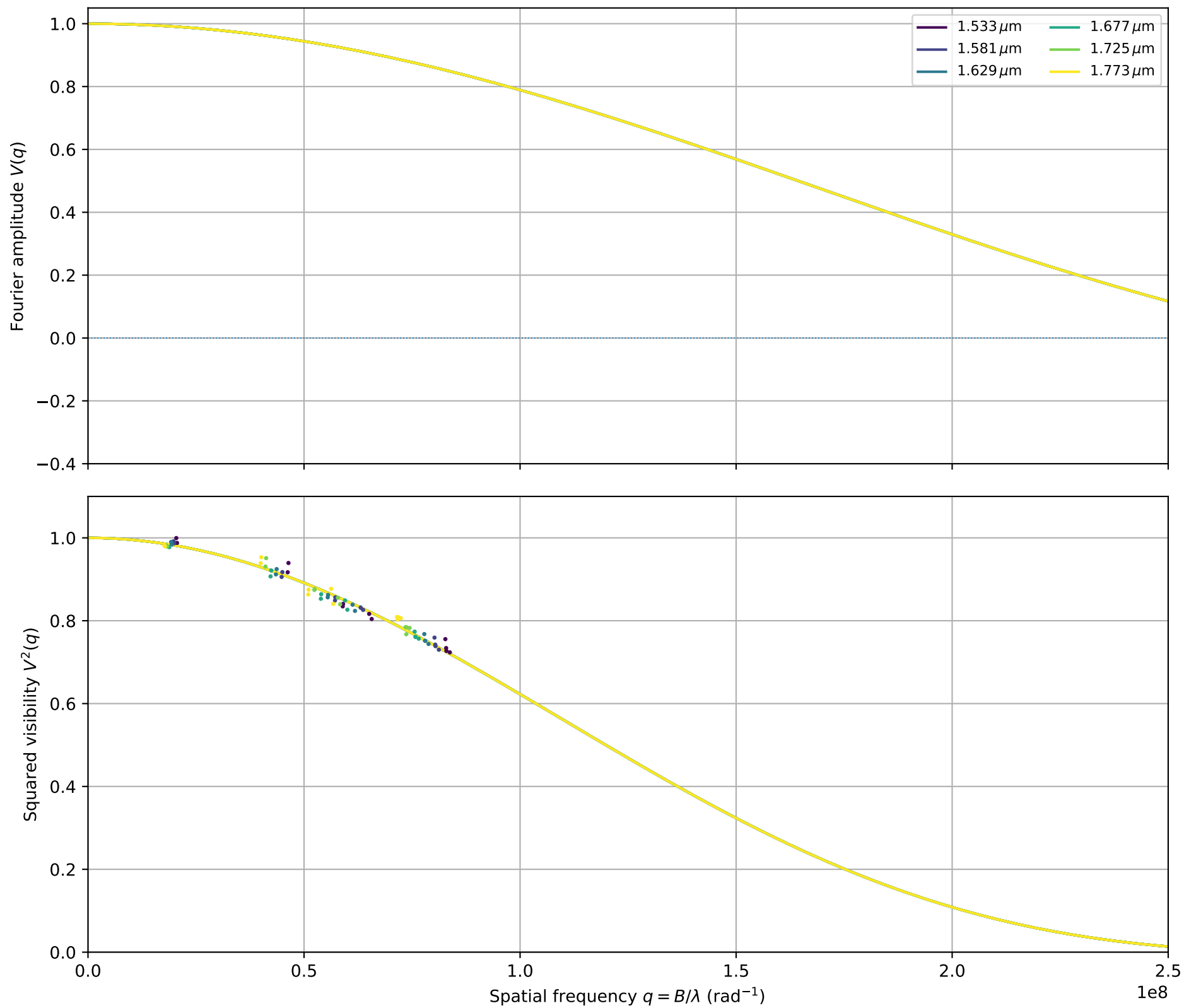
psi Vel A: fitted \theta_{\text{LDD}} = 0.8990 \pm 0.0001 mas
