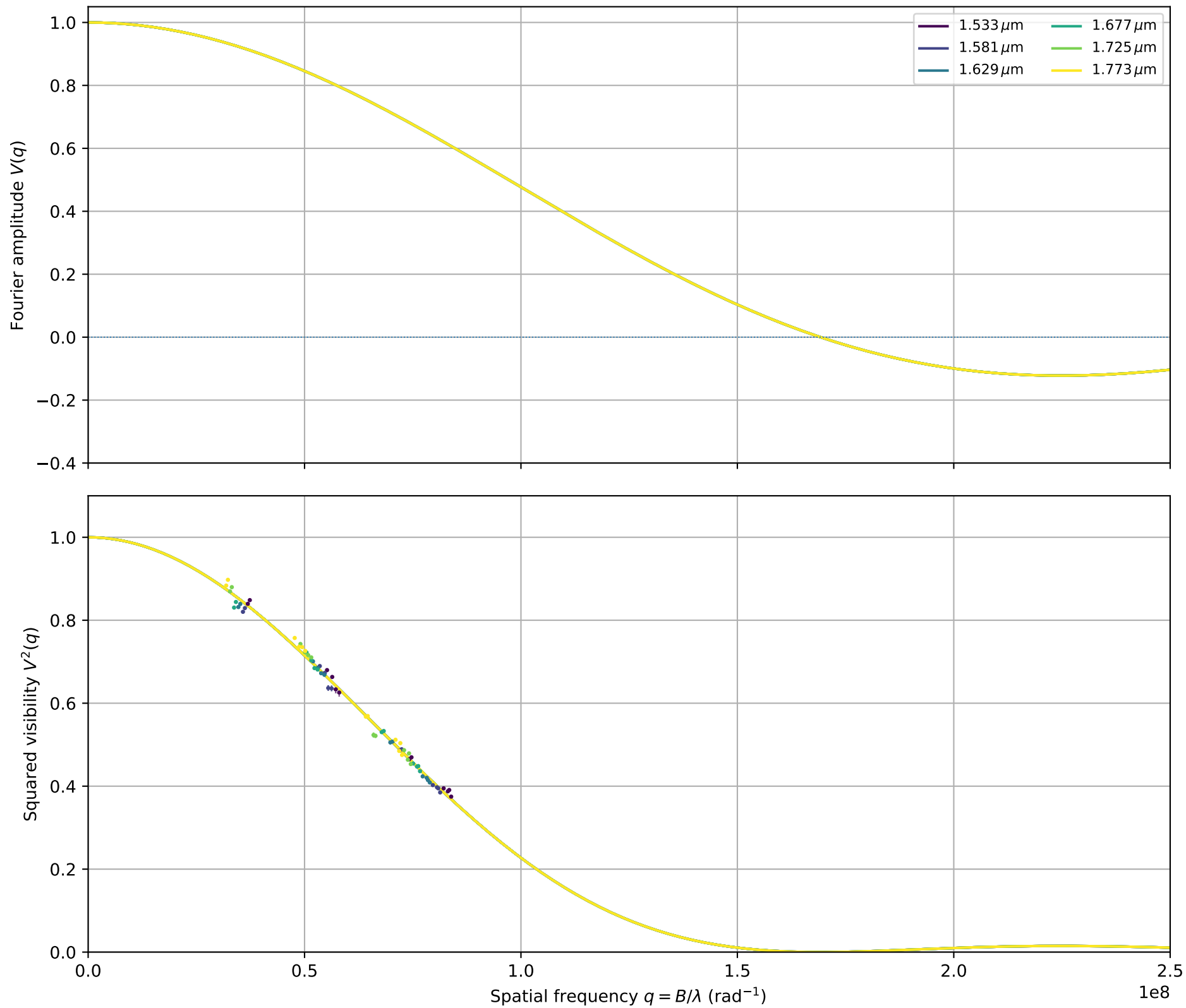
pi3_Ori: fitted \theta_{\text{LDD}} = 1.5245 \pm 0.0037 mas
