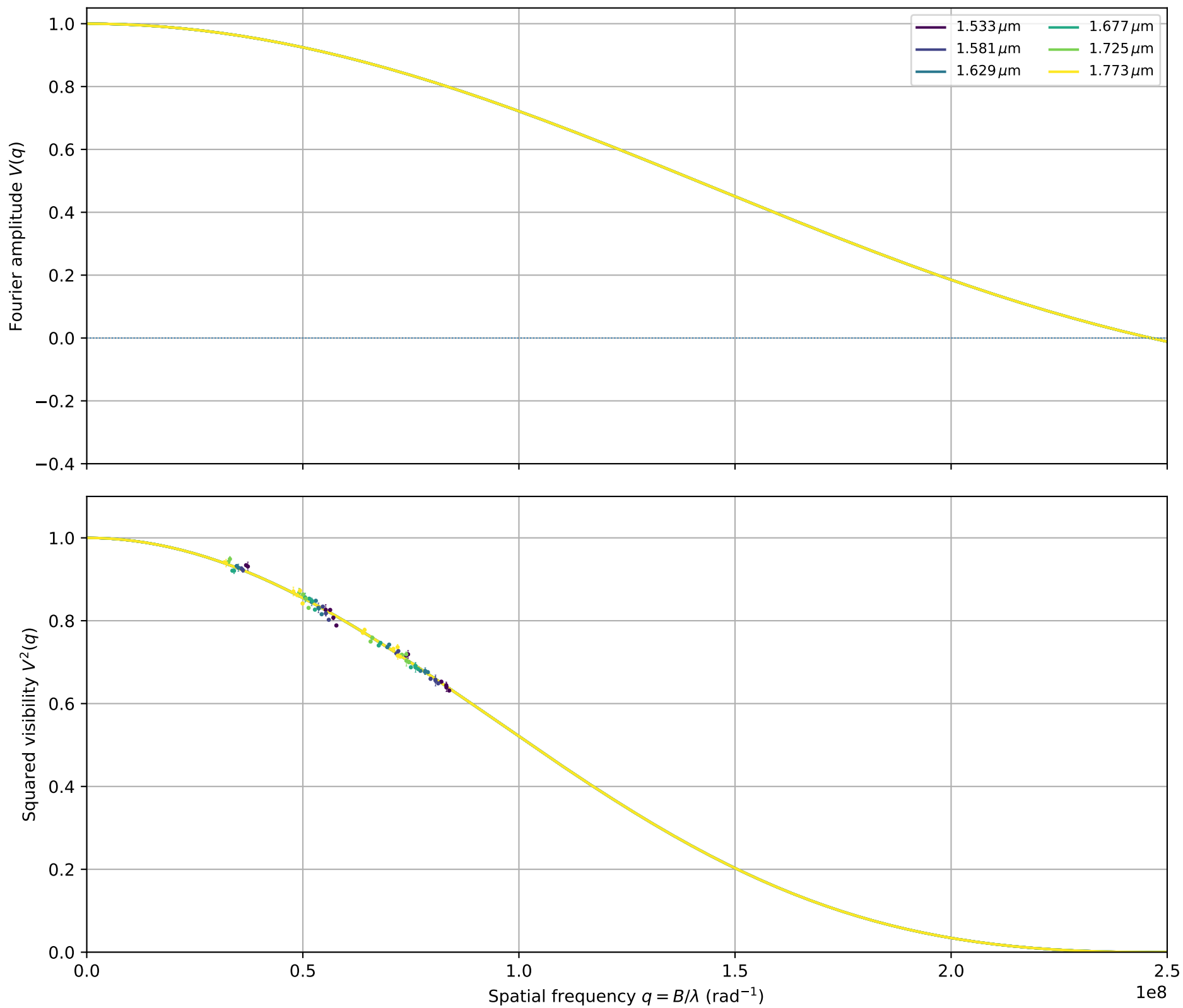
HD141004: fitted \theta_{\text{LDD}} = 1.0526 \pm 0.0003 mas
