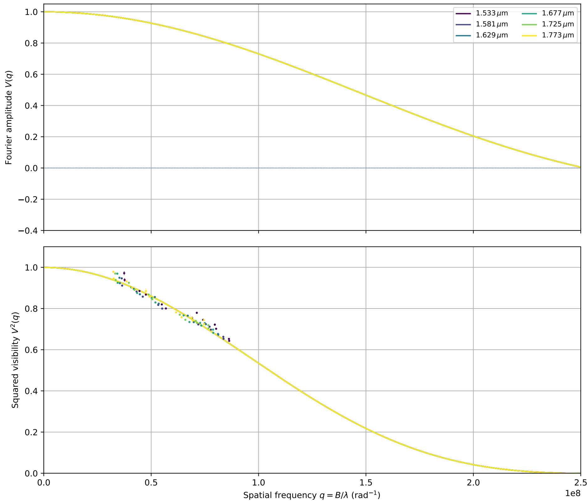
HR_2998: fitted \theta_{\text{LDD}} = 1.0421 \pm 0.0001 mas
