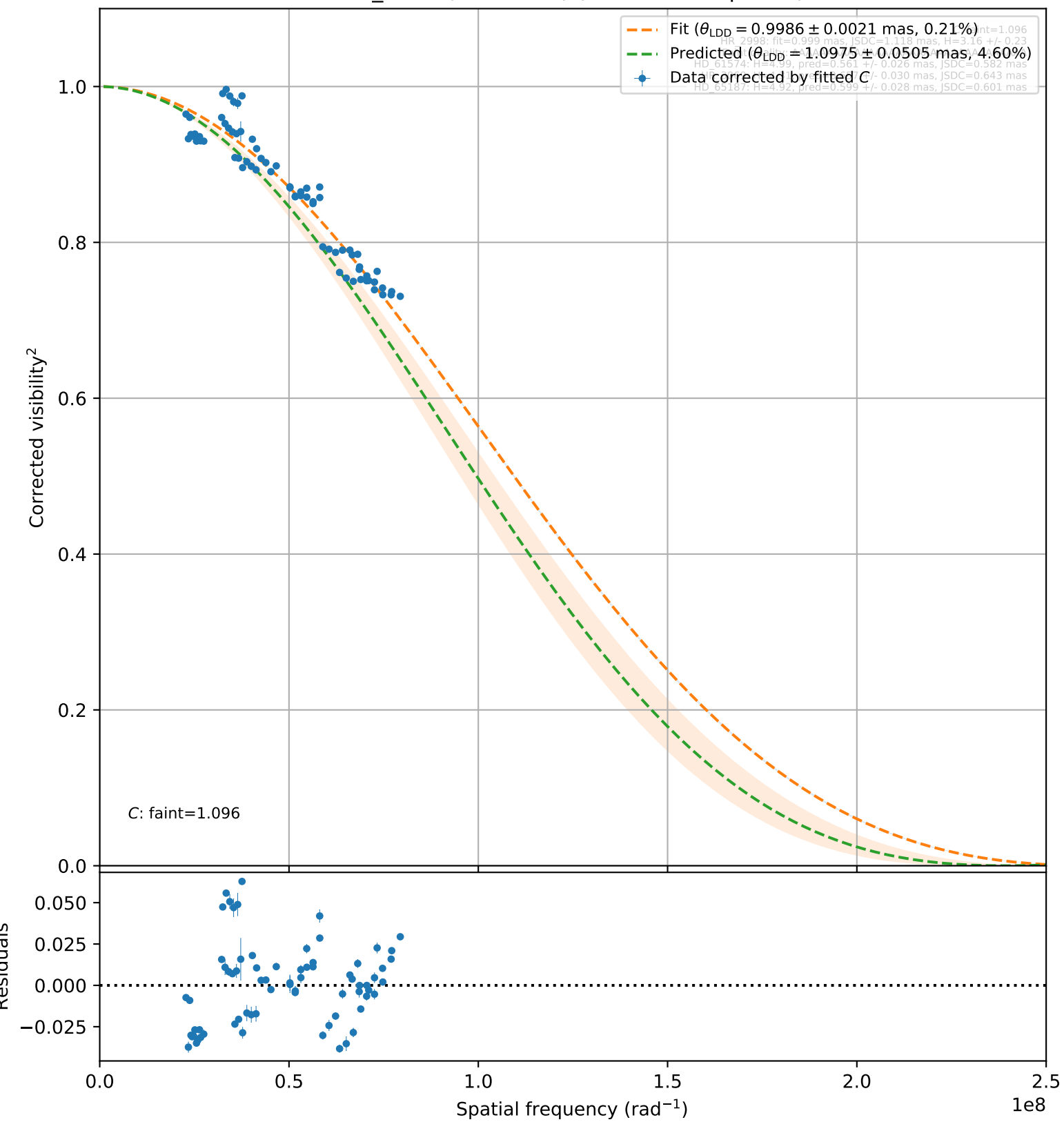
HR_2998 (faint, 104) (72 valid vis 2 points)
