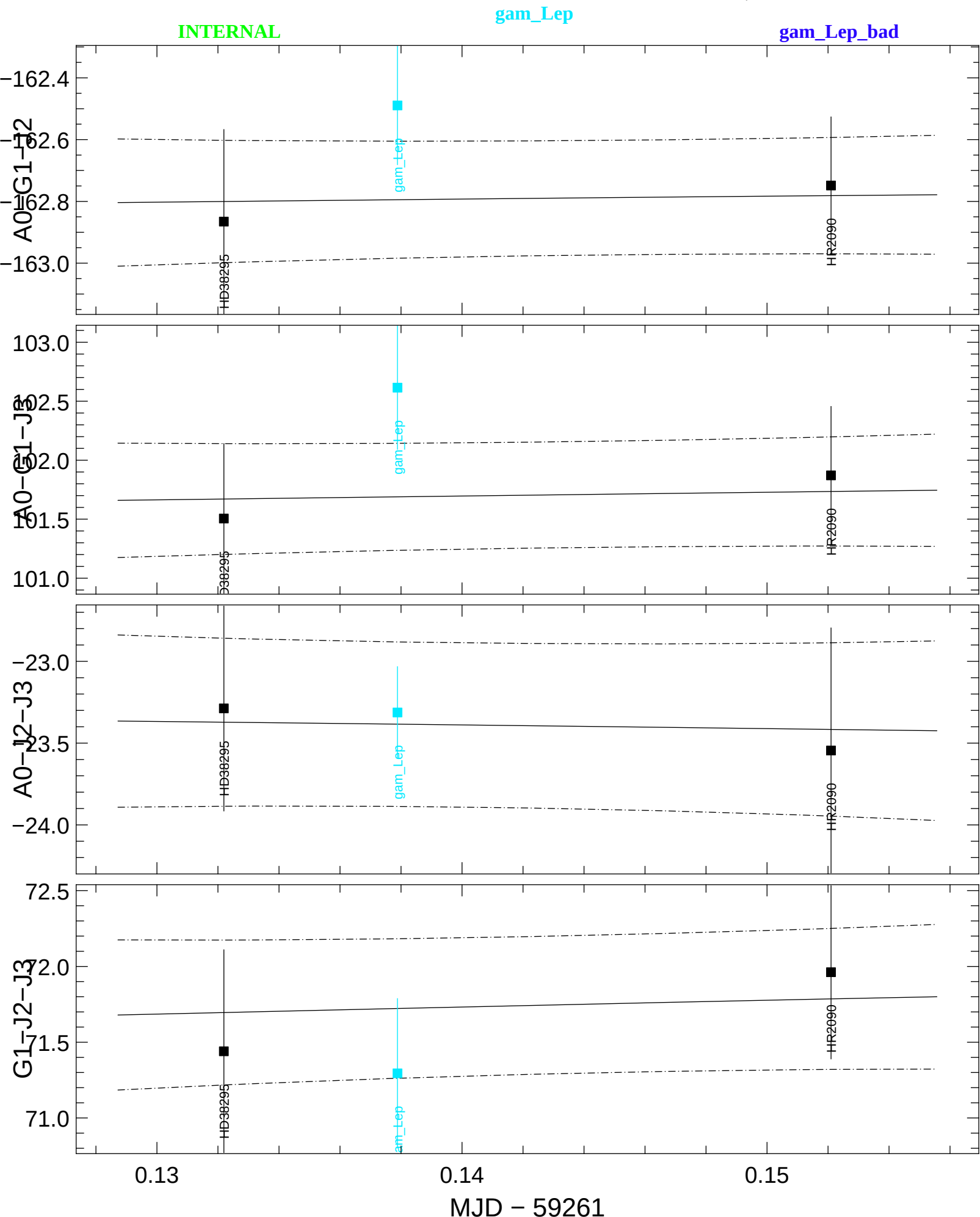
Transfer-Function t3Phi (black) and Scientific t3Phi (colors) averaged in the range [1.61995,1.61995] \mu m
