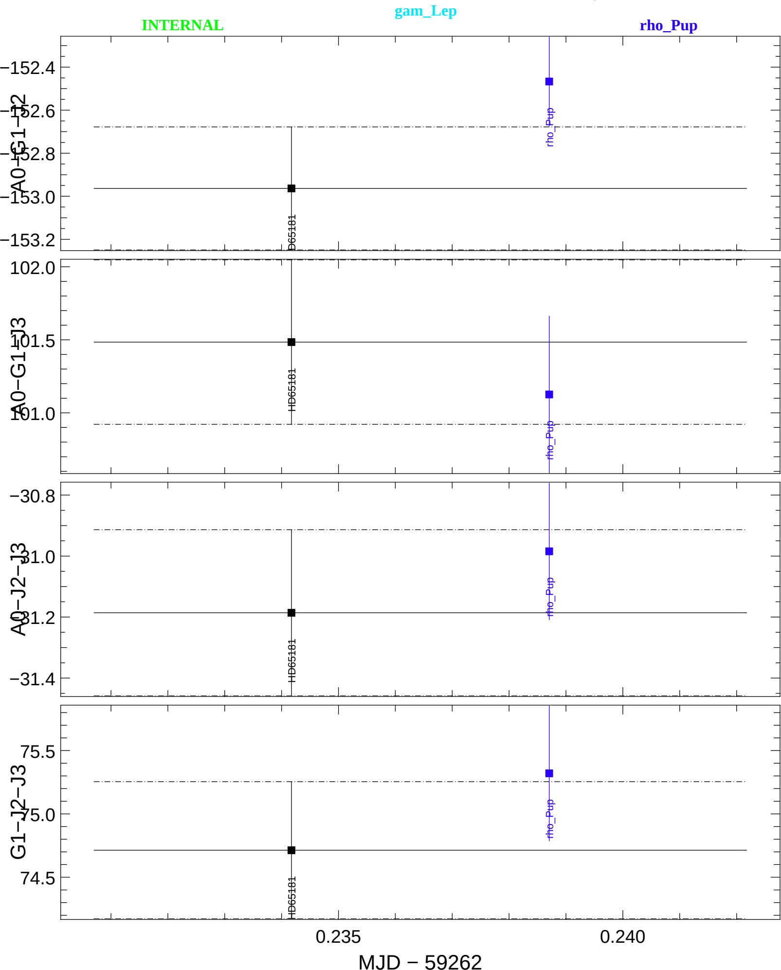
Transfer-Function t3Phi (black) and Scientific t3Phi (colors) averaged in the range [1.61907,1.61907] \mu m
