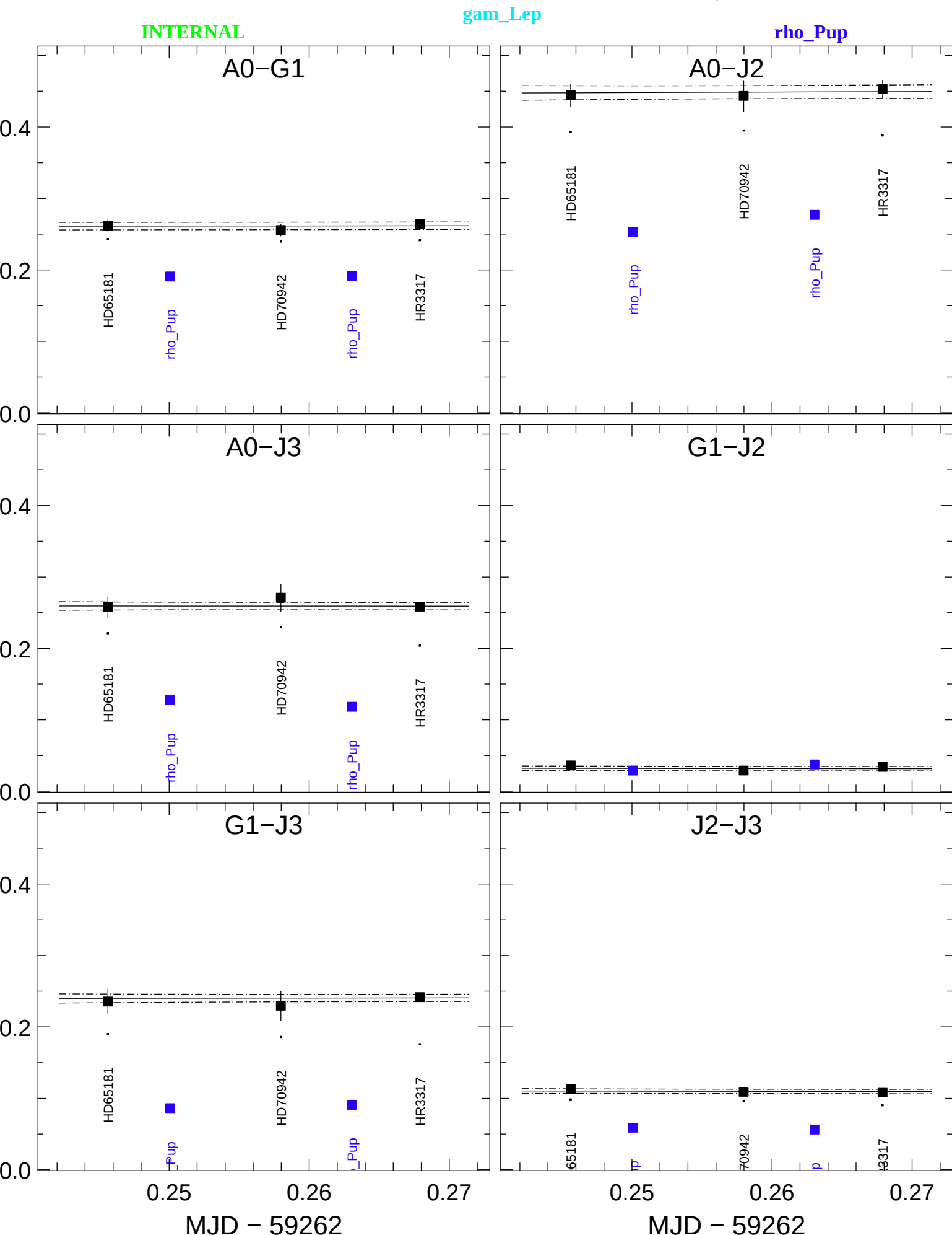
Transfer-Function vis2 (black) and Scientific vis2 (colors) averaged in the range [1.61907,1.61907] \mu m
