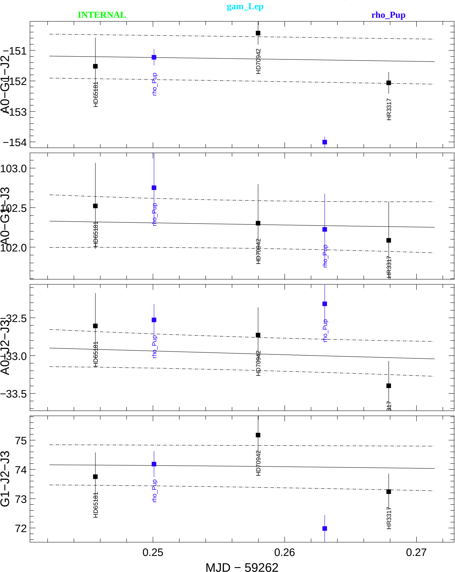
Transfer-Function t3Phi (black) and Scientific t3Phi (colors) averaged in the range [1.61907,1.61907] \mu\text{m}
