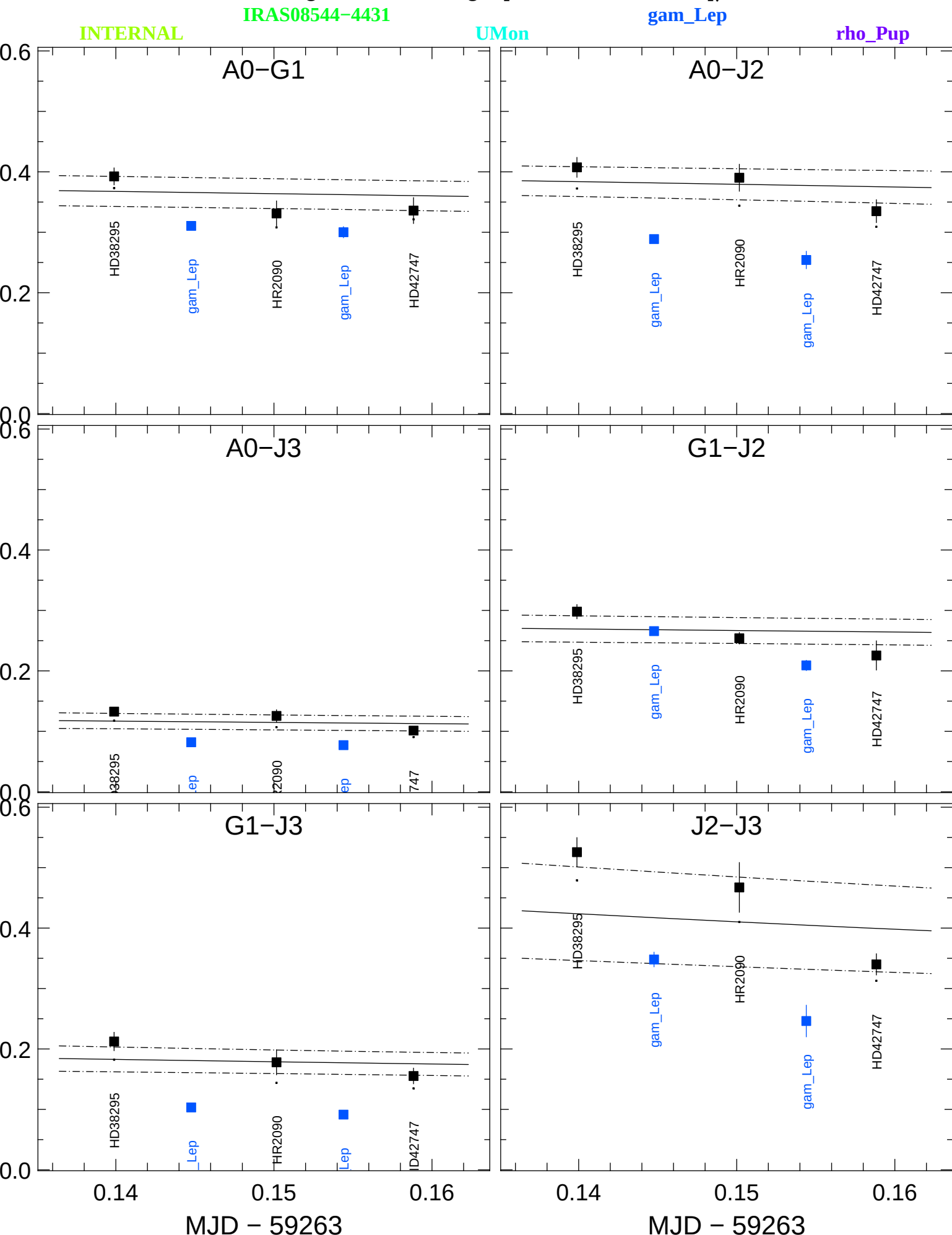
Transfer-Function vis2 (black) and Scientific vis2 (colors) averaged in the range [1.62139,1.62139] \mu\text{m}
