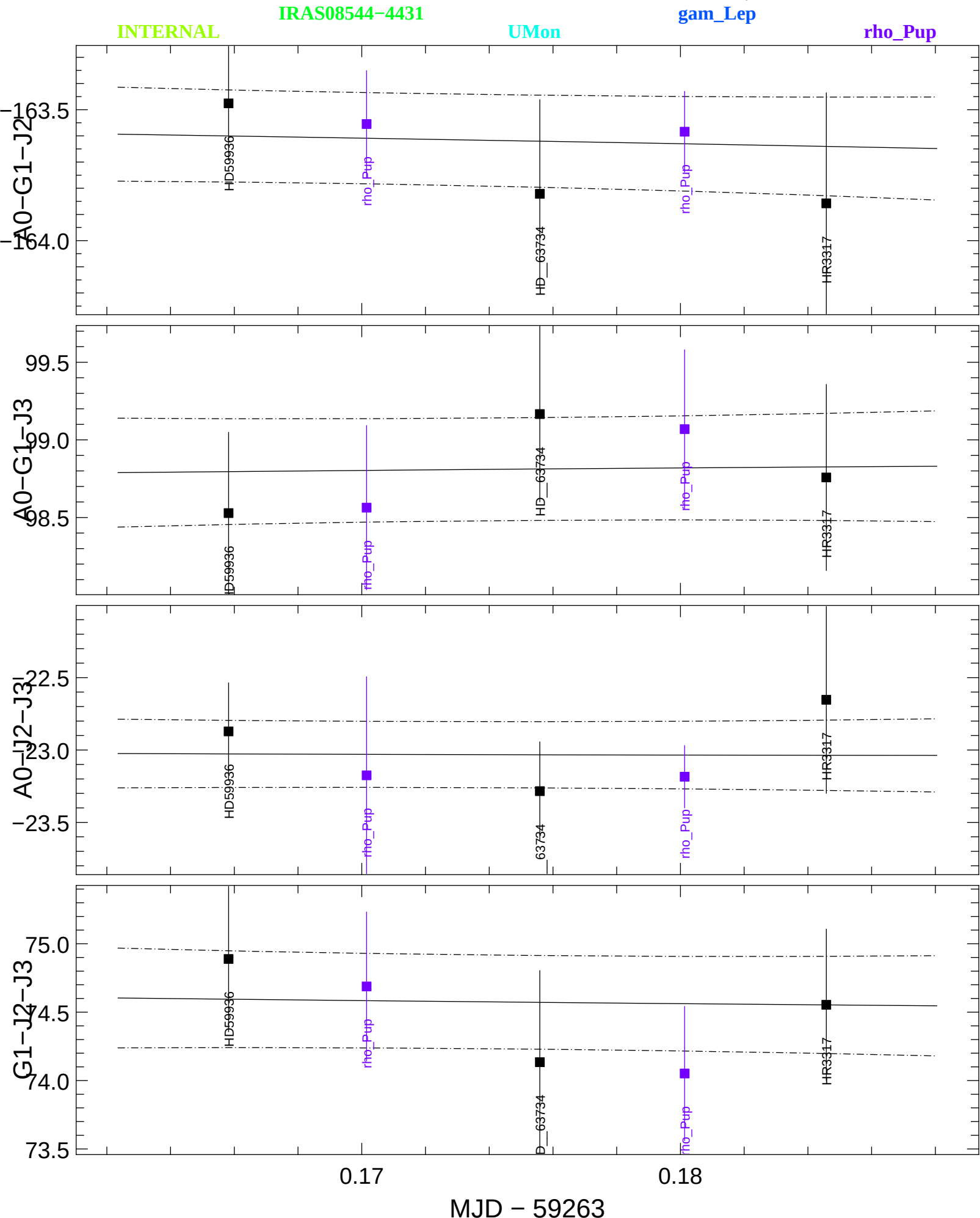
Transfer-Function t3Phi (black) and Scientific t3Phi (colors) averaged in the range [1.62139,1.62139] \mu m
