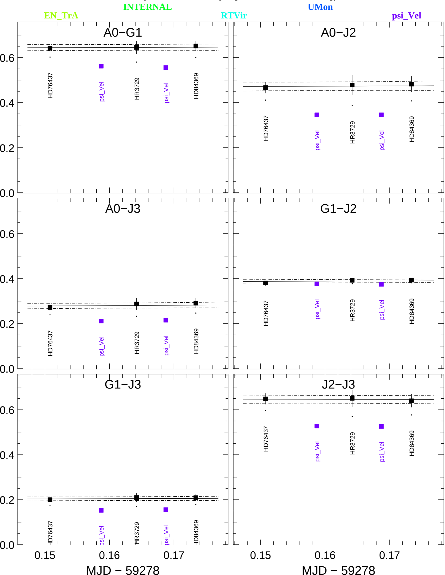
Transfer-Function vis2 (black) and Scientific vis2 (colors) averaged in the range [1.61887,1.61887] \mu\text{m}
