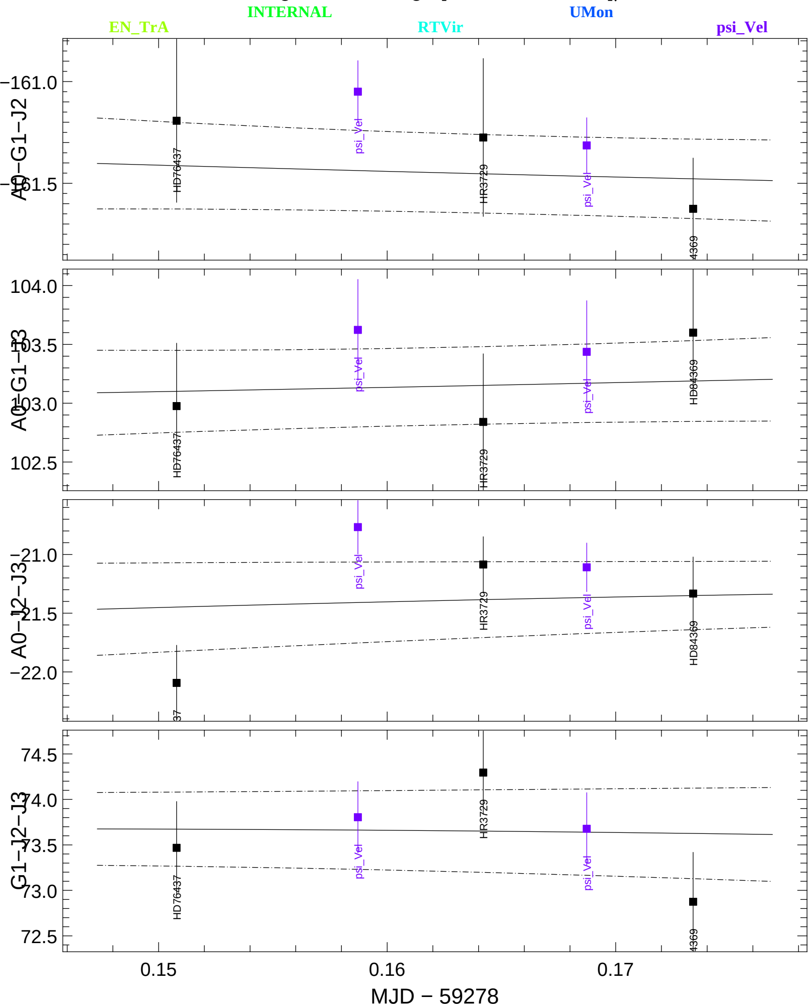
Transfer-Function t3Phi (black) and Scientific t3Phi (colors) averaged in the range [1.61887,1.61887] \mu m
