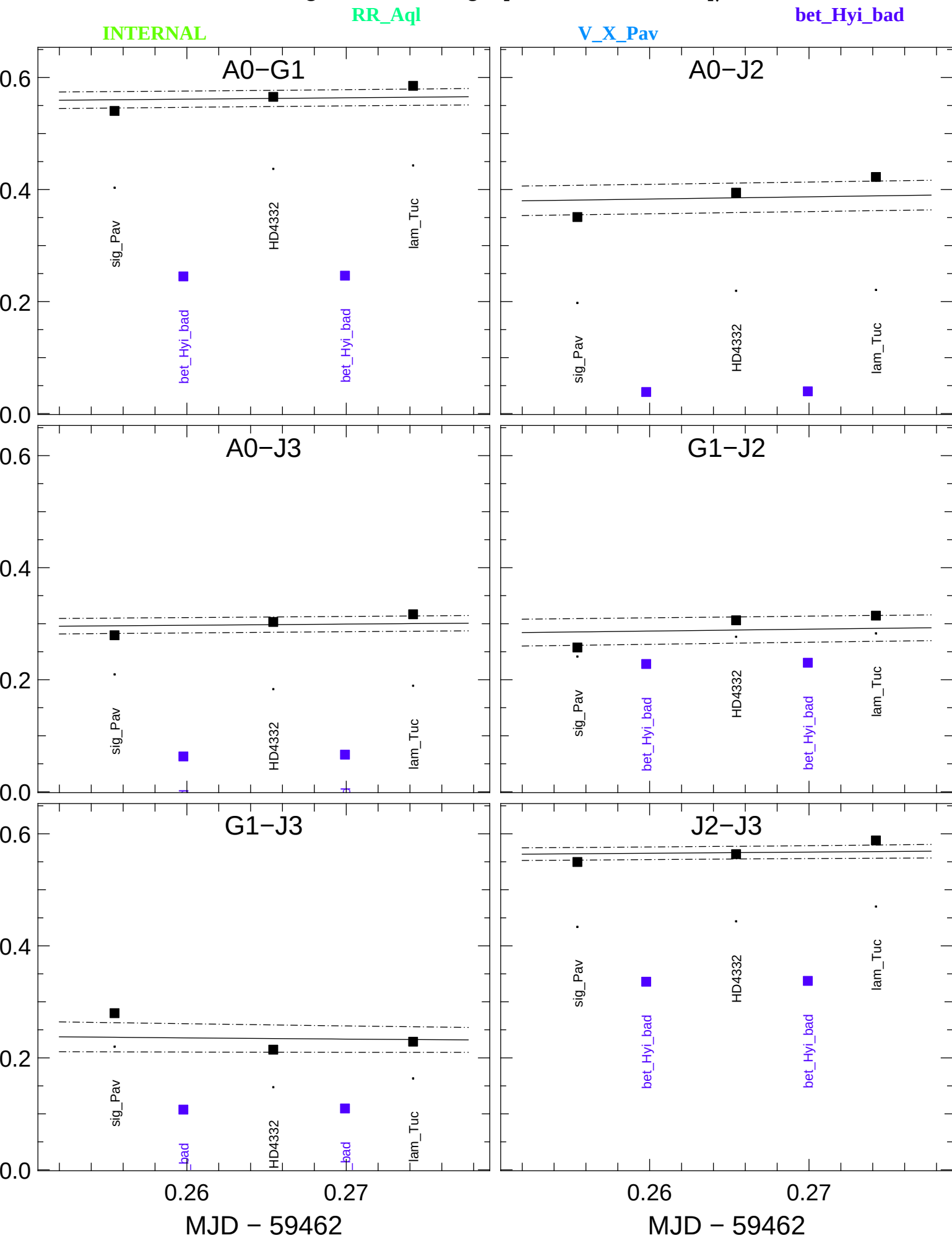
Transfer-Function vis2 (black) and Scientific vis2 (colors) averaged in the range [1.61549,1.61549] \mu\text{m}
