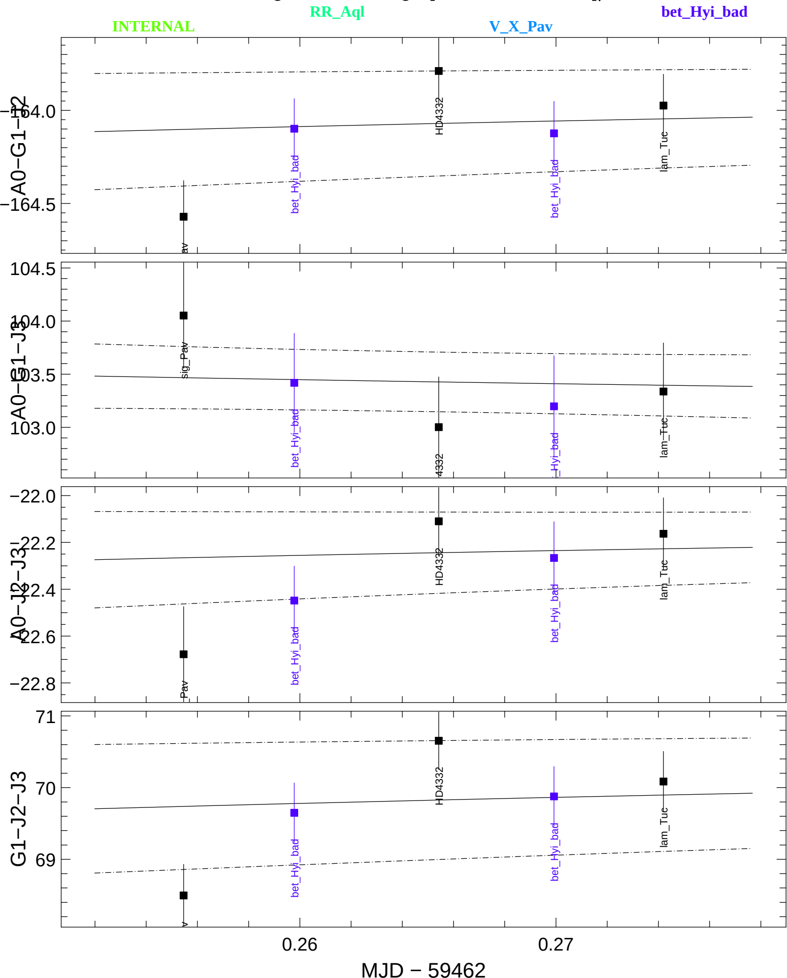
Transfer-Function t3Phi (black) and Scientific t3Phi (colors) averaged in the range [1.61549,1.61549] \mu m
