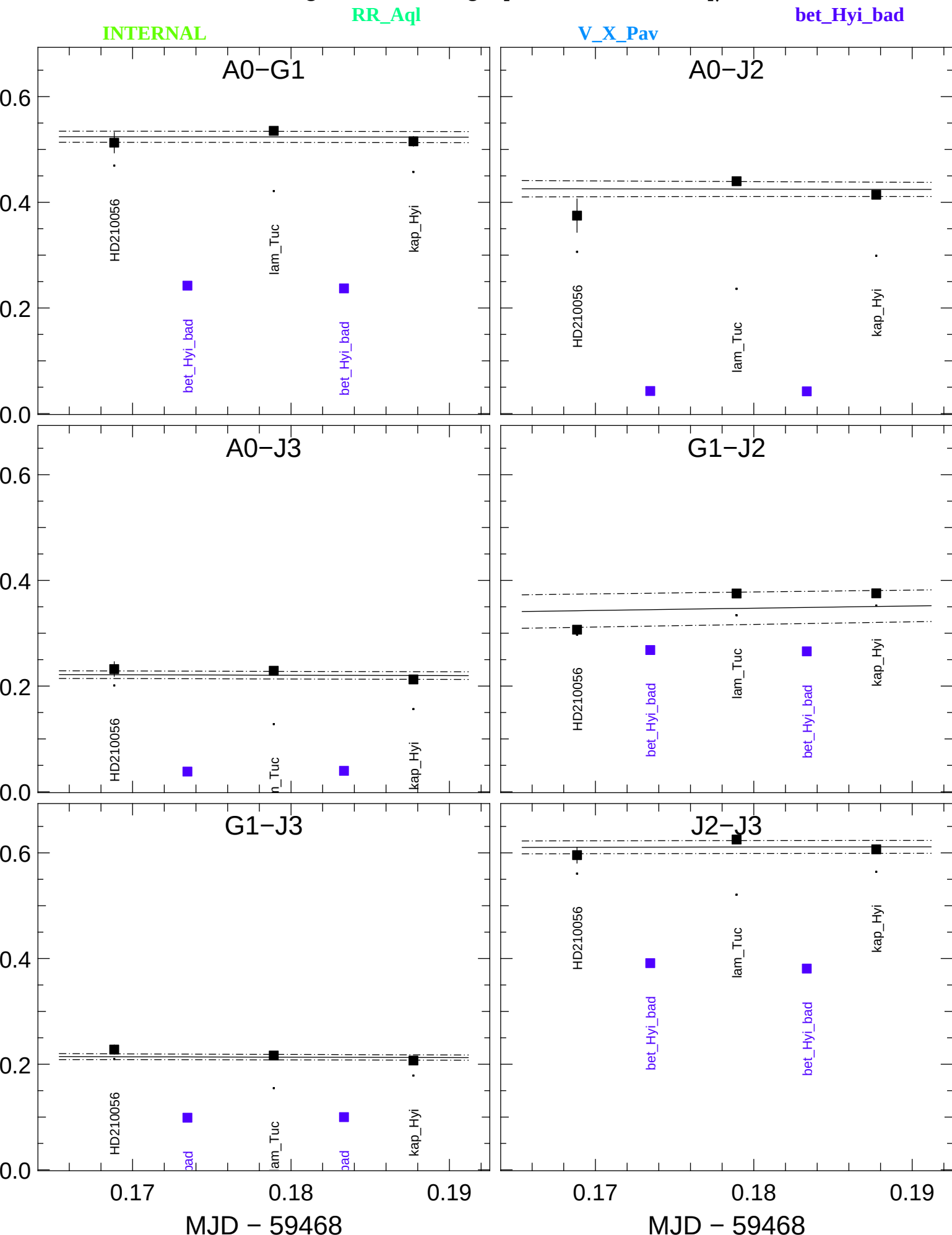
Transfer-Function vis2 (black) and Scientific vis2 (colors) averaged in the range [1.61397,1.61397] \mu\text{m}
