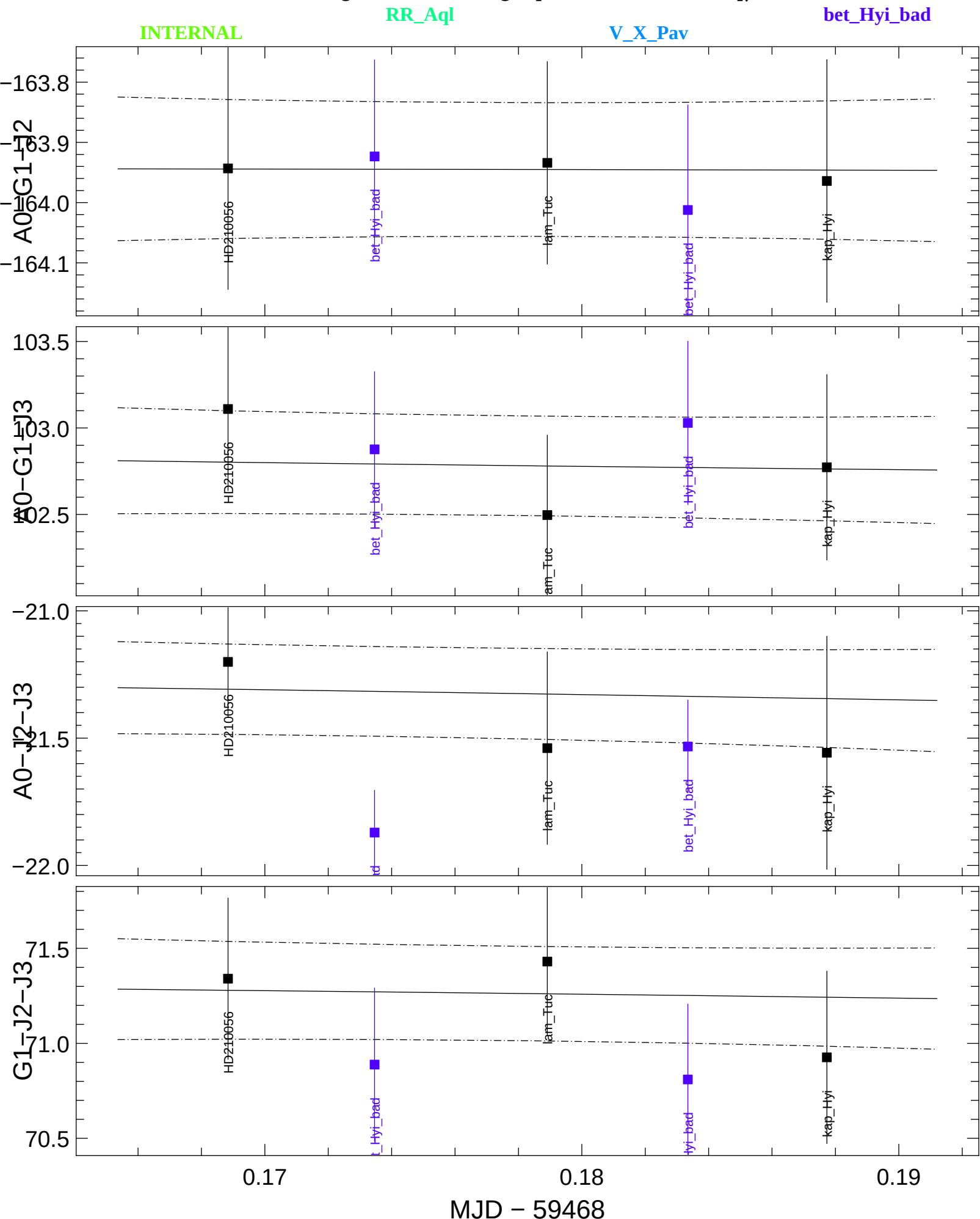
Transfer-Function t3Phi (black) and Scientific t3Phi (colors) averaged in the range [1.61397,1.61397] \mu m
