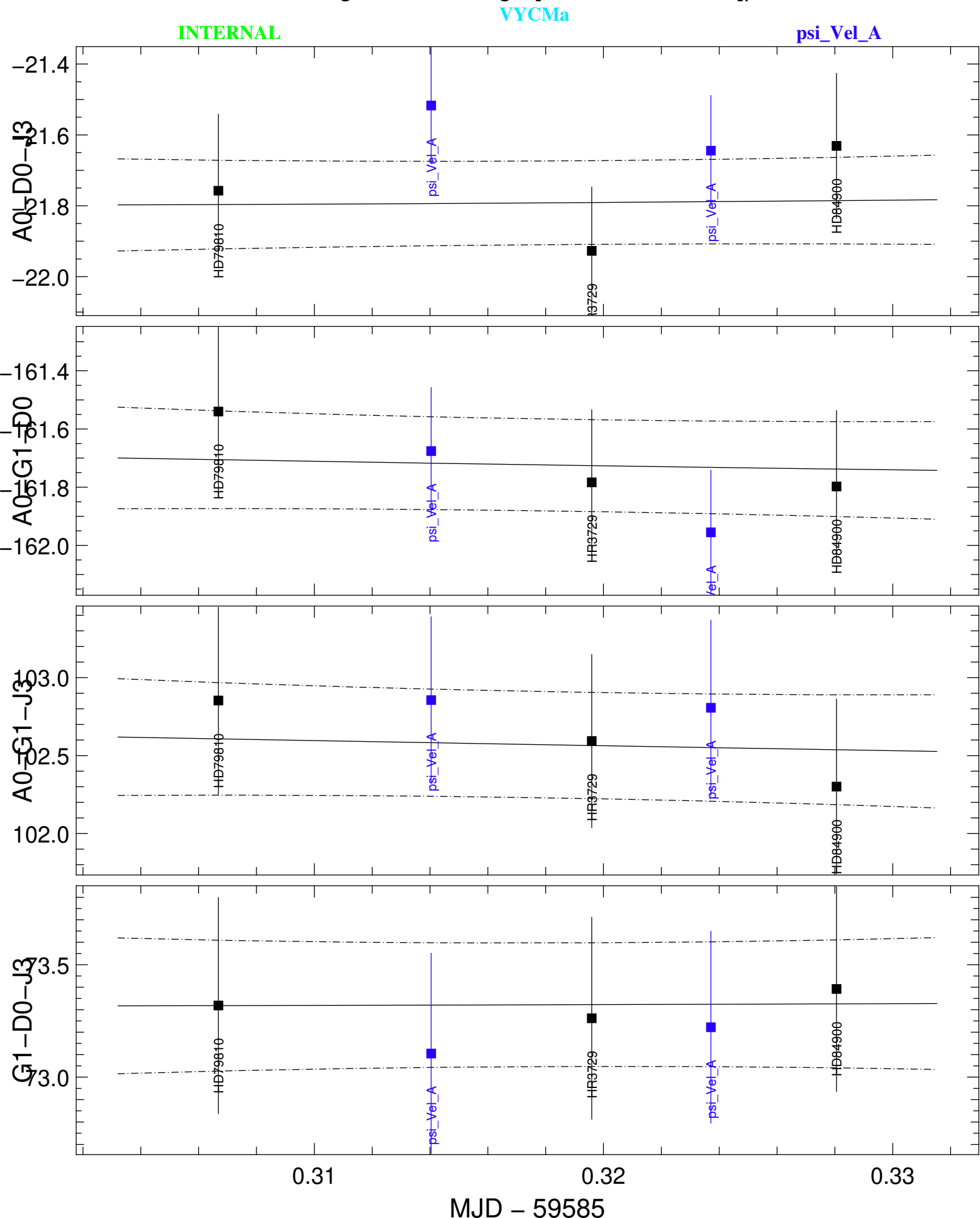
Transfer-Function t3Phi (black) and Scientific t3Phi (colors) averaged in the range [1.61956,1.61956] \mu m
