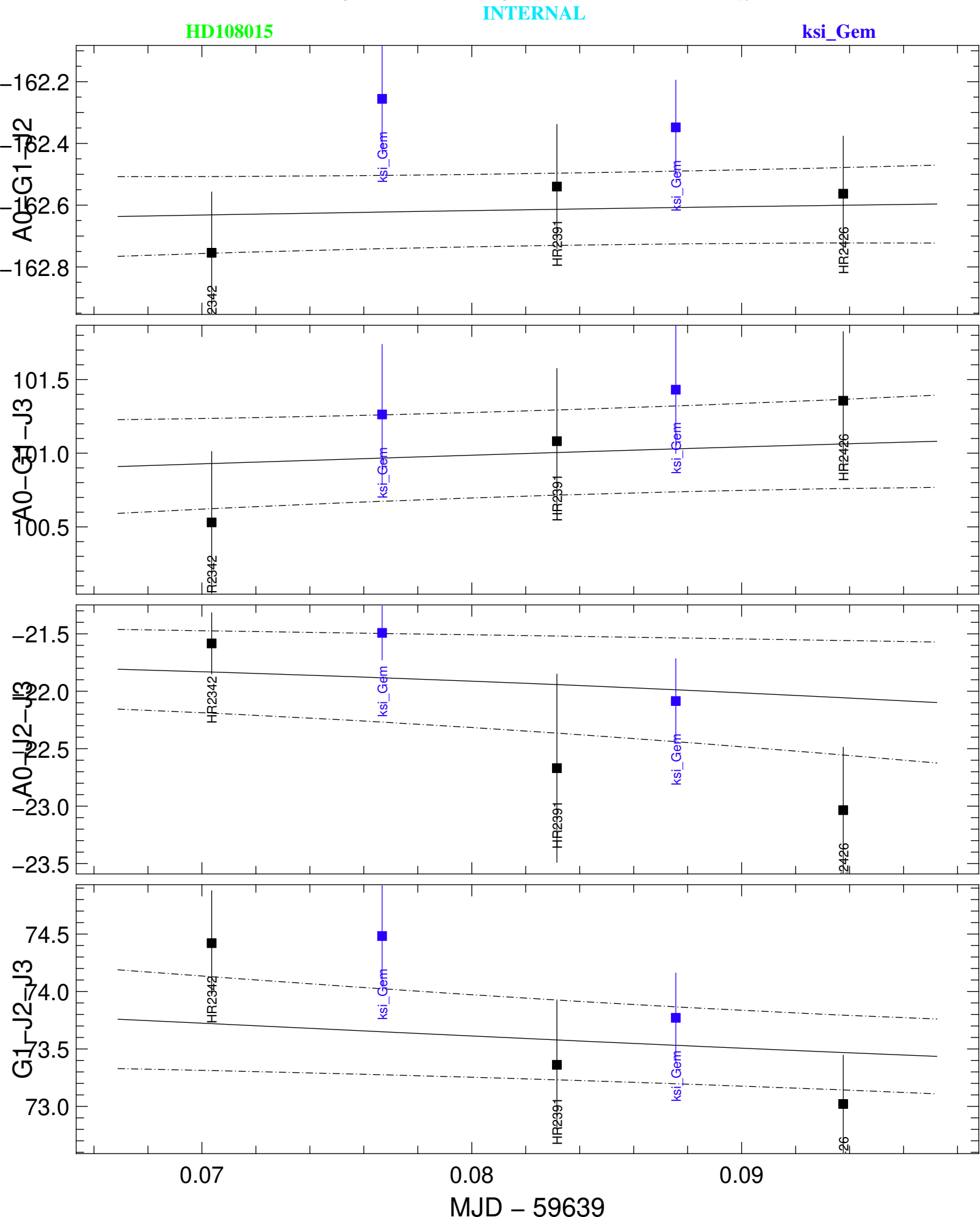
Transfer-Function t3Phi (black) and Scientific t3Phi (colors) averaged in the range [1.62229,1.62229] \mu m
