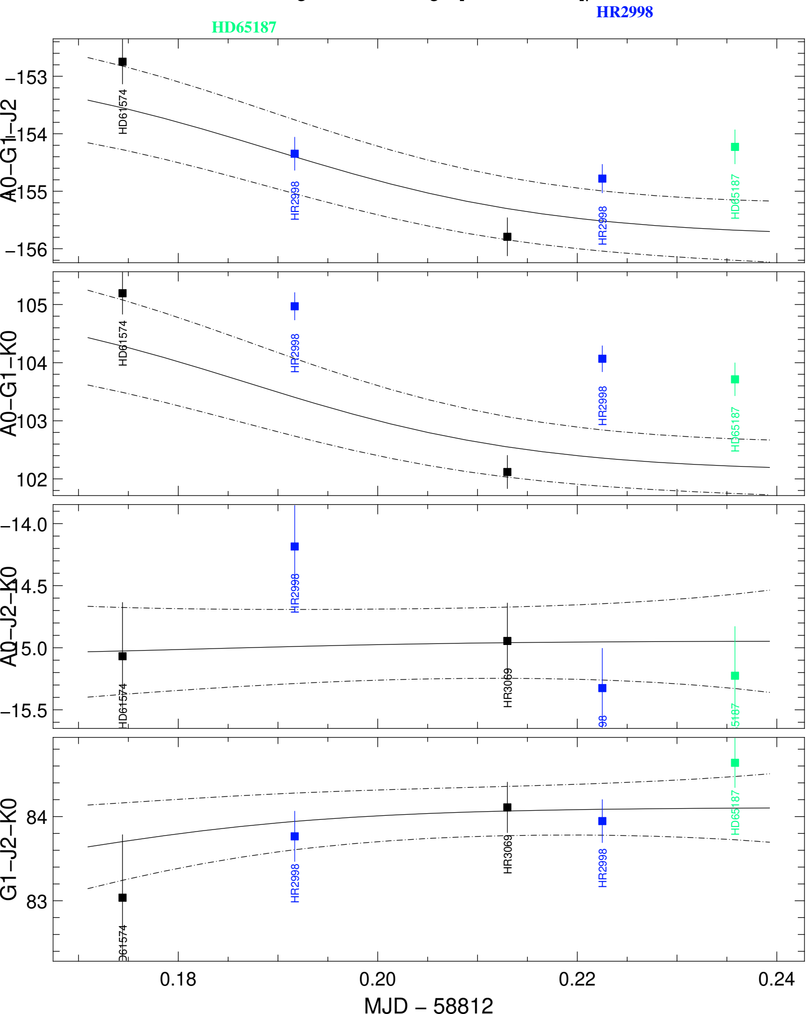
Transfer-Function t3Phi (black) and Scientific t3Phi (colors) averaged in the range [1.581,1.581] \mu m
