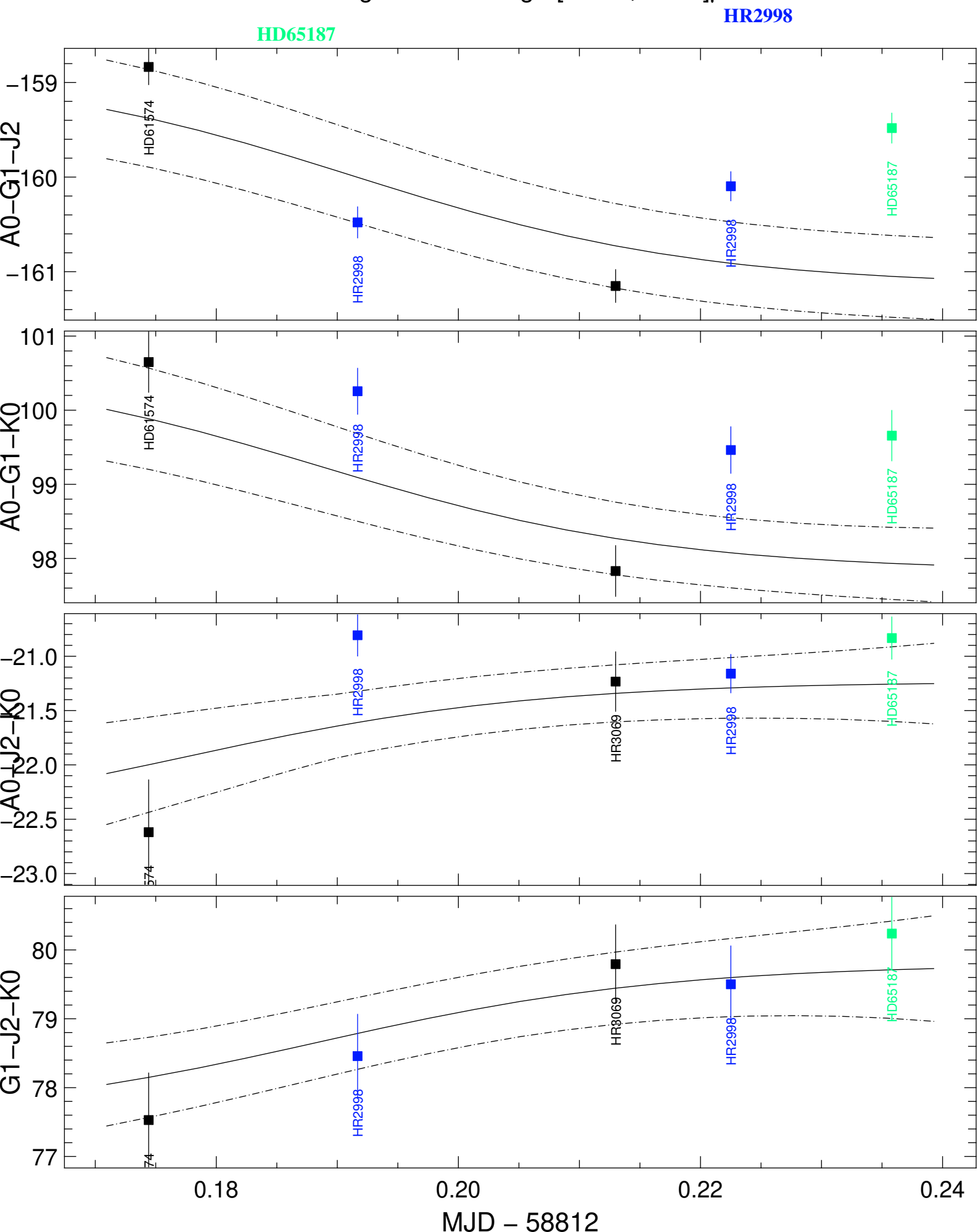
Transfer-Function t3Phi (black) and Scientific t3Phi (colors) averaged in the range [1.677,1.677] \mu m
