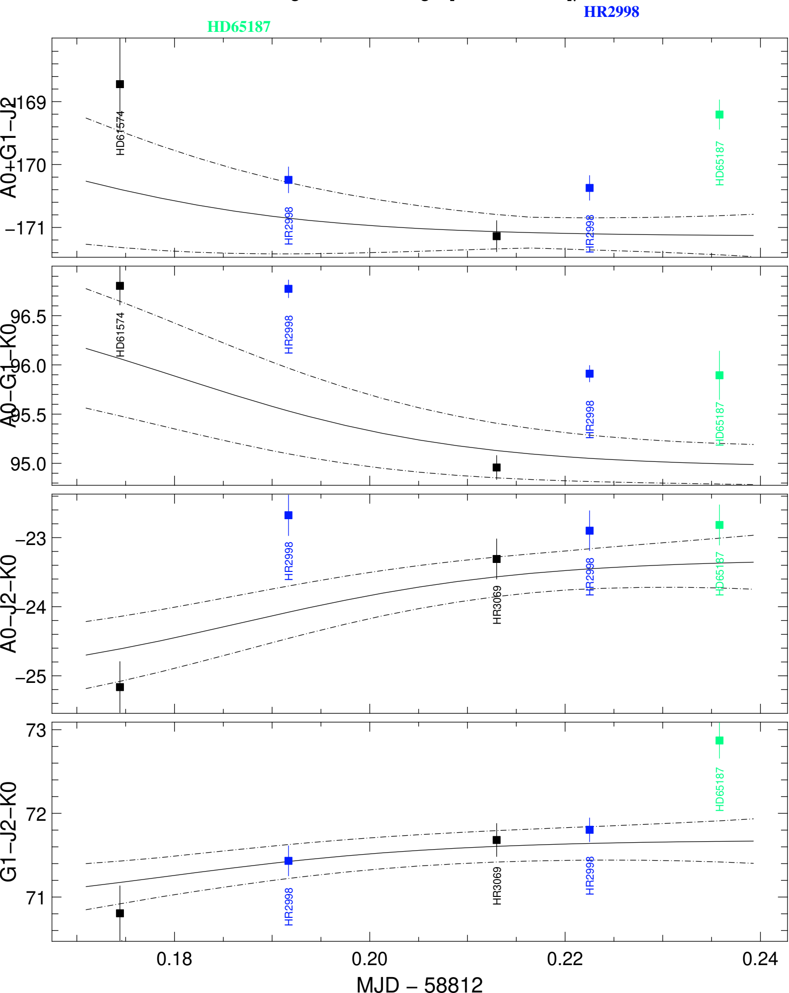
Transfer-Function t3Phi (black) and Scientific t3Phi (colors) averaged in the range [1.725,1.725] \mu m
