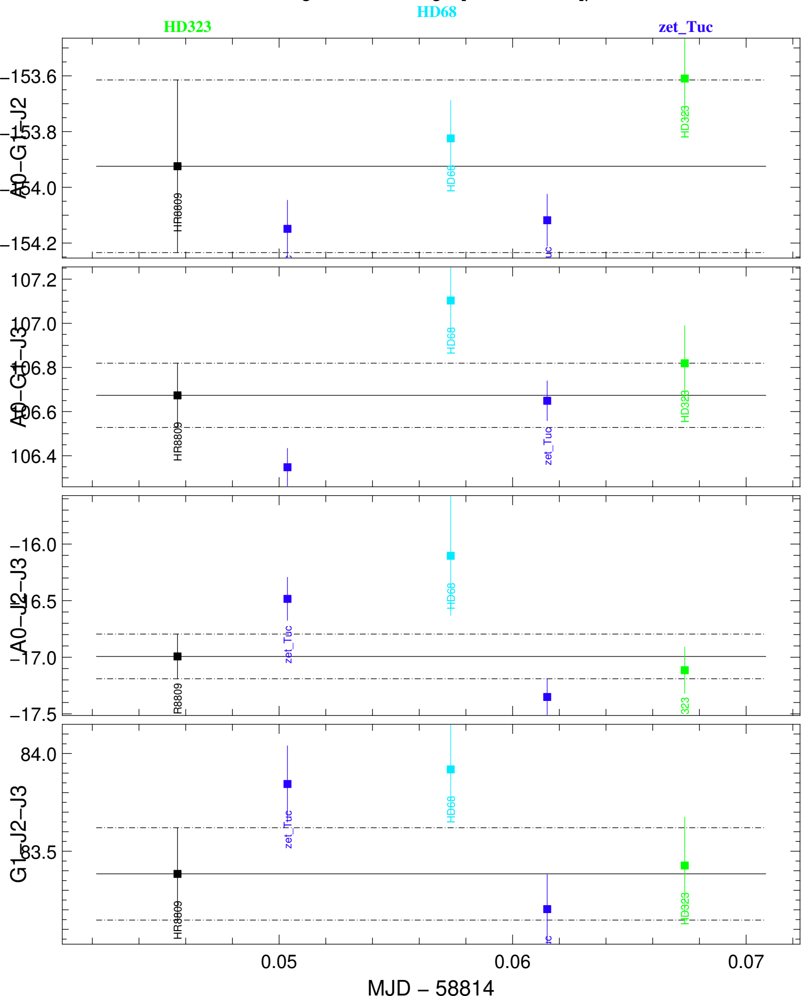
Transfer-Function t3Phi (black) and Scientific t3Phi (colors) averaged in the range [1.533,1.533] \mu m
