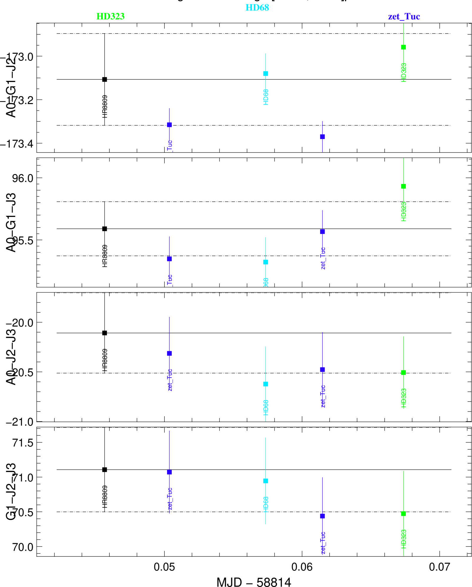
Transfer-Function t3Phi (black) and Scientific t3Phi (colors) averaged in the range [1.773,1.773] \mu m
