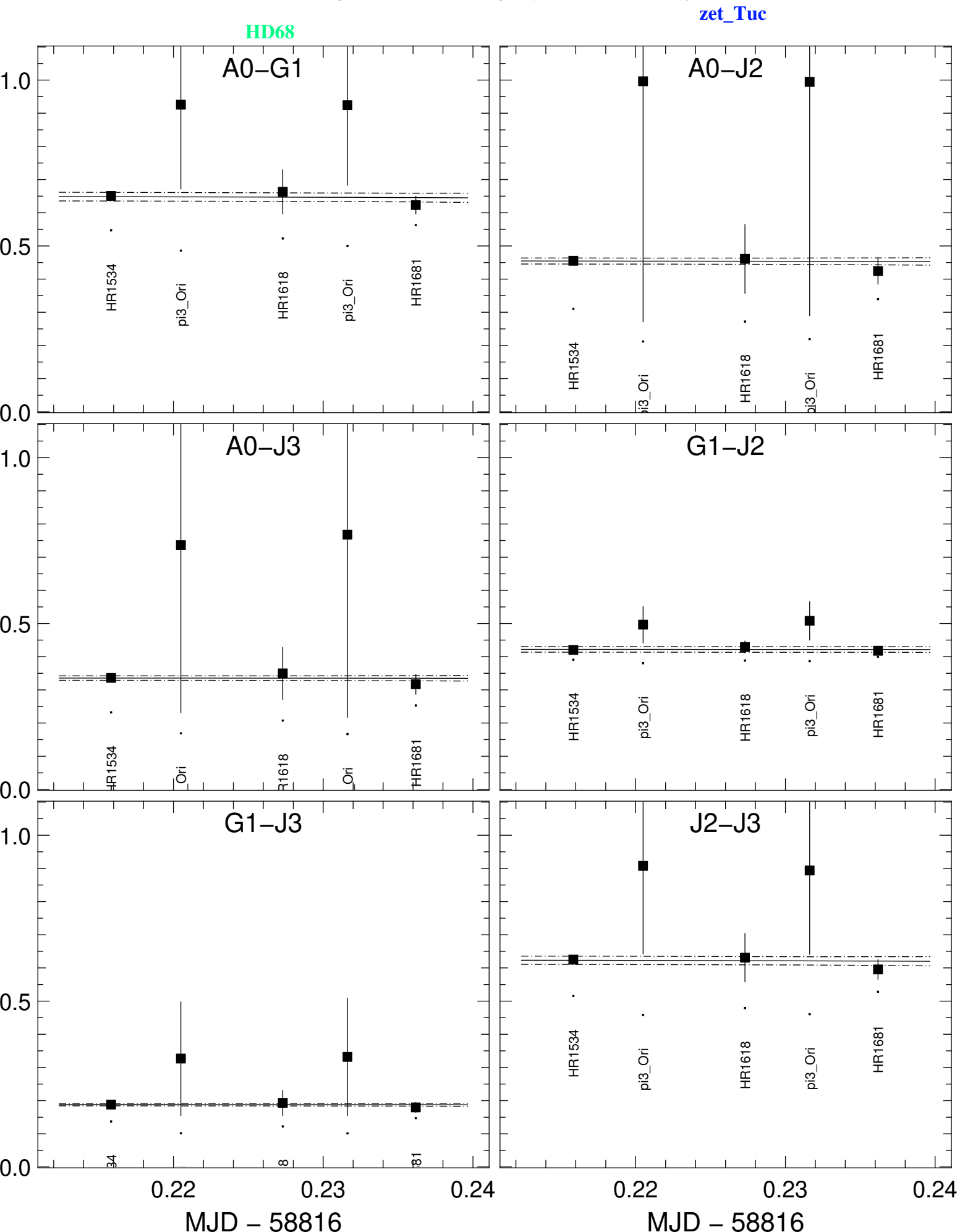
Transfer-Function vis2 (black) and Scientific vis2 (colors) averaged in the range [1.725, 1.725]\mu\text{m}
