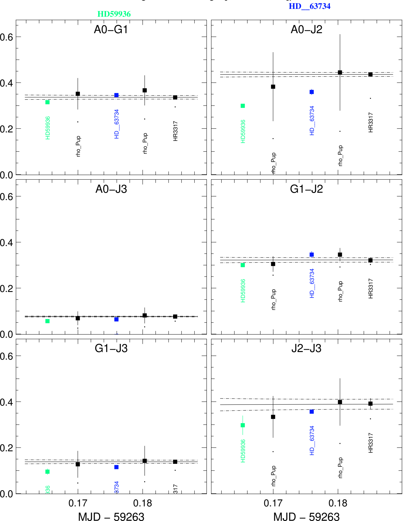
Transfer-Function vis2 (black) and Scientific vis2 (colors) averaged in the range [1.629,1.629] \mu m
