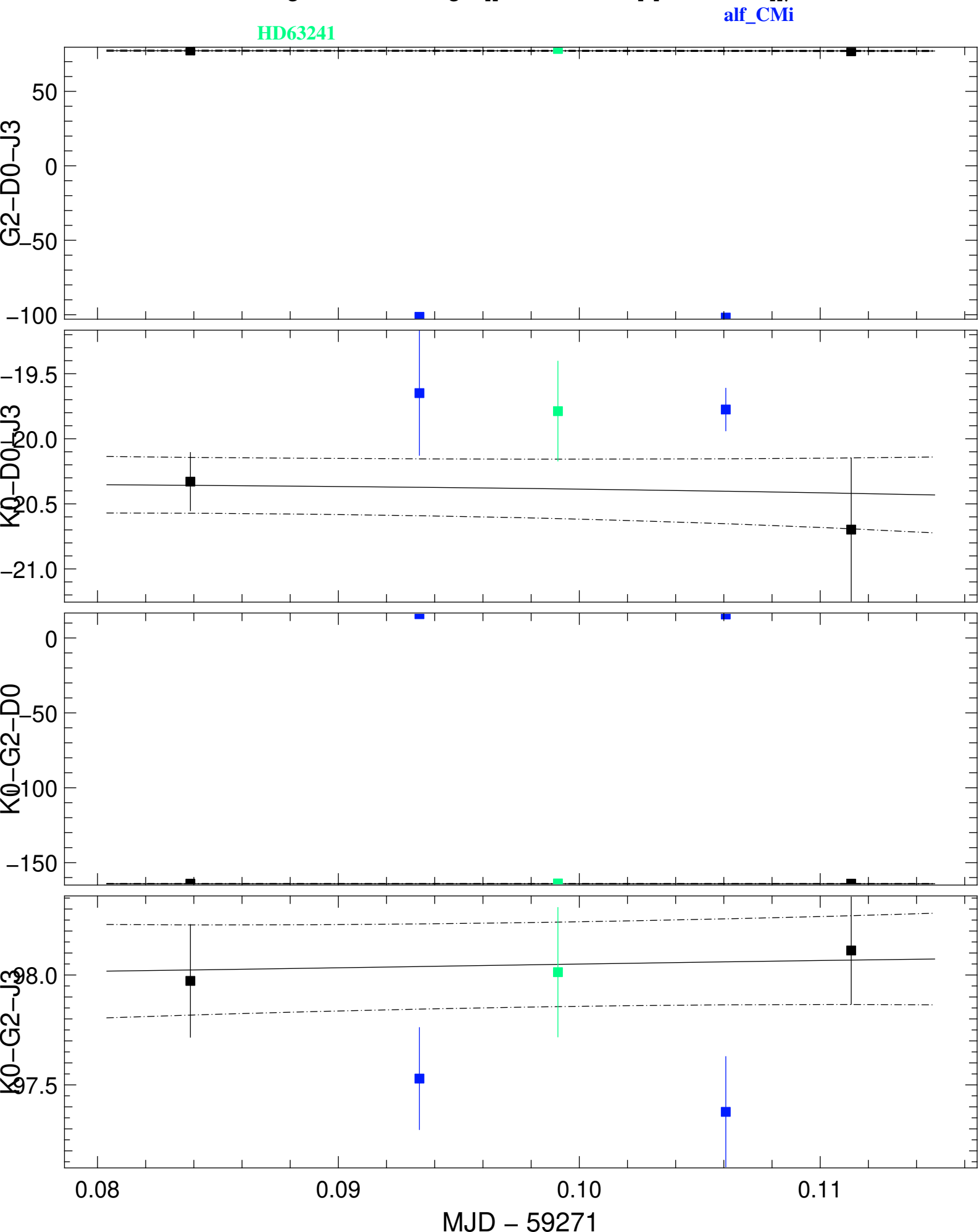
Transfer-Function t3Phi (black) and Scientific t3Phi (colors) averaged in the range [[1.637, 1.715], [2.04, 2.25]]\mu\text{m}
