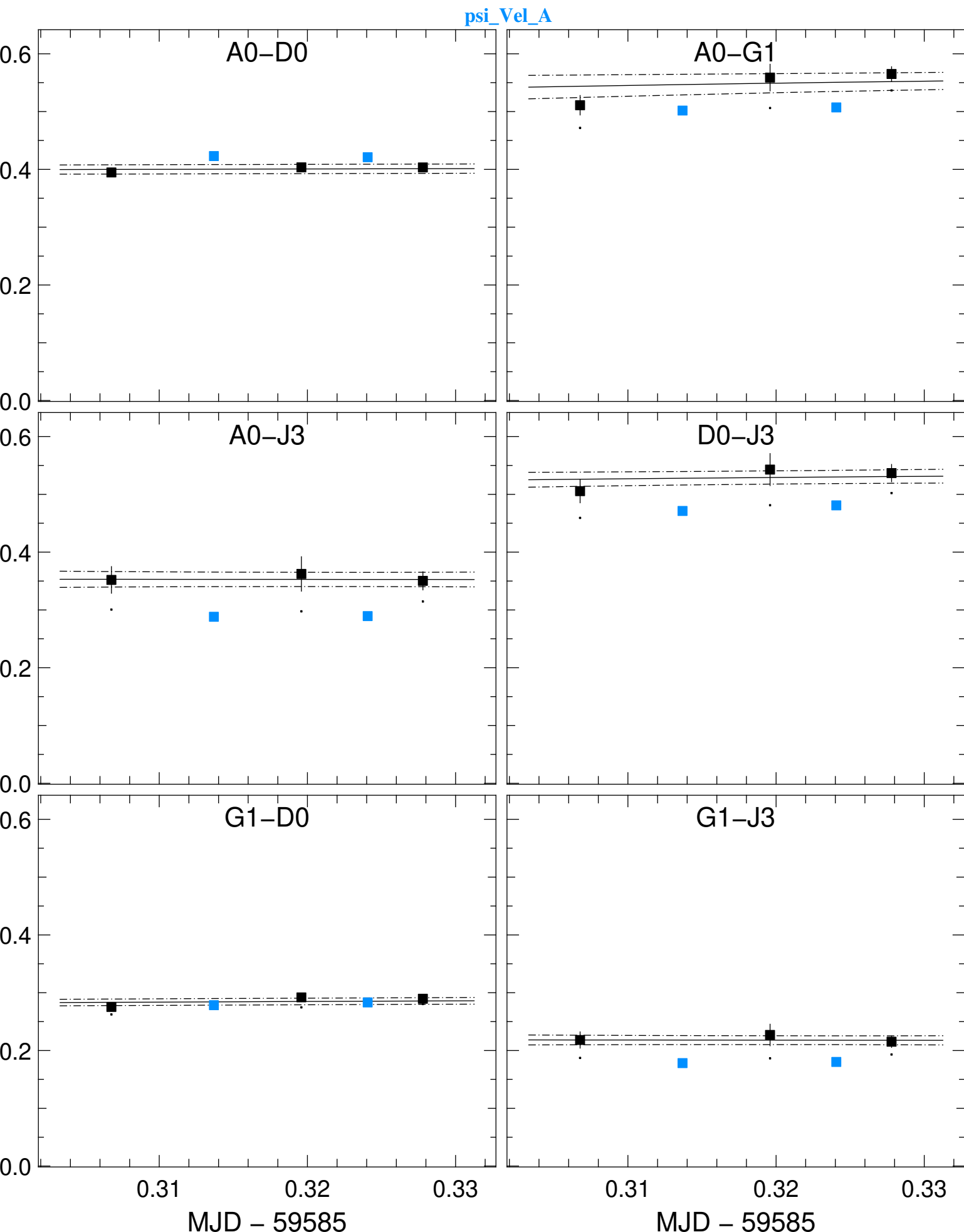
Transfer-Function vis2 (black) and Scientific vis2 (colors) averaged in the range [[1.637, 1.715], [2.04, 2.25]] \mu\text{m}
