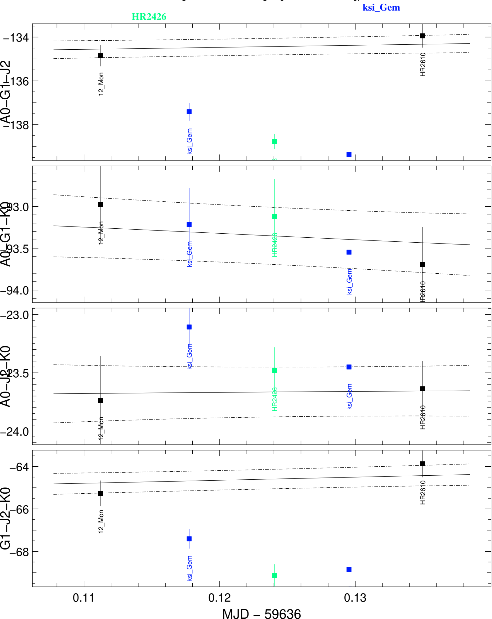
Transfer-Function t3Phi (black) and Scientific t3Phi (colors) averaged in the range [1.629,1.629] \mu\text{m}
