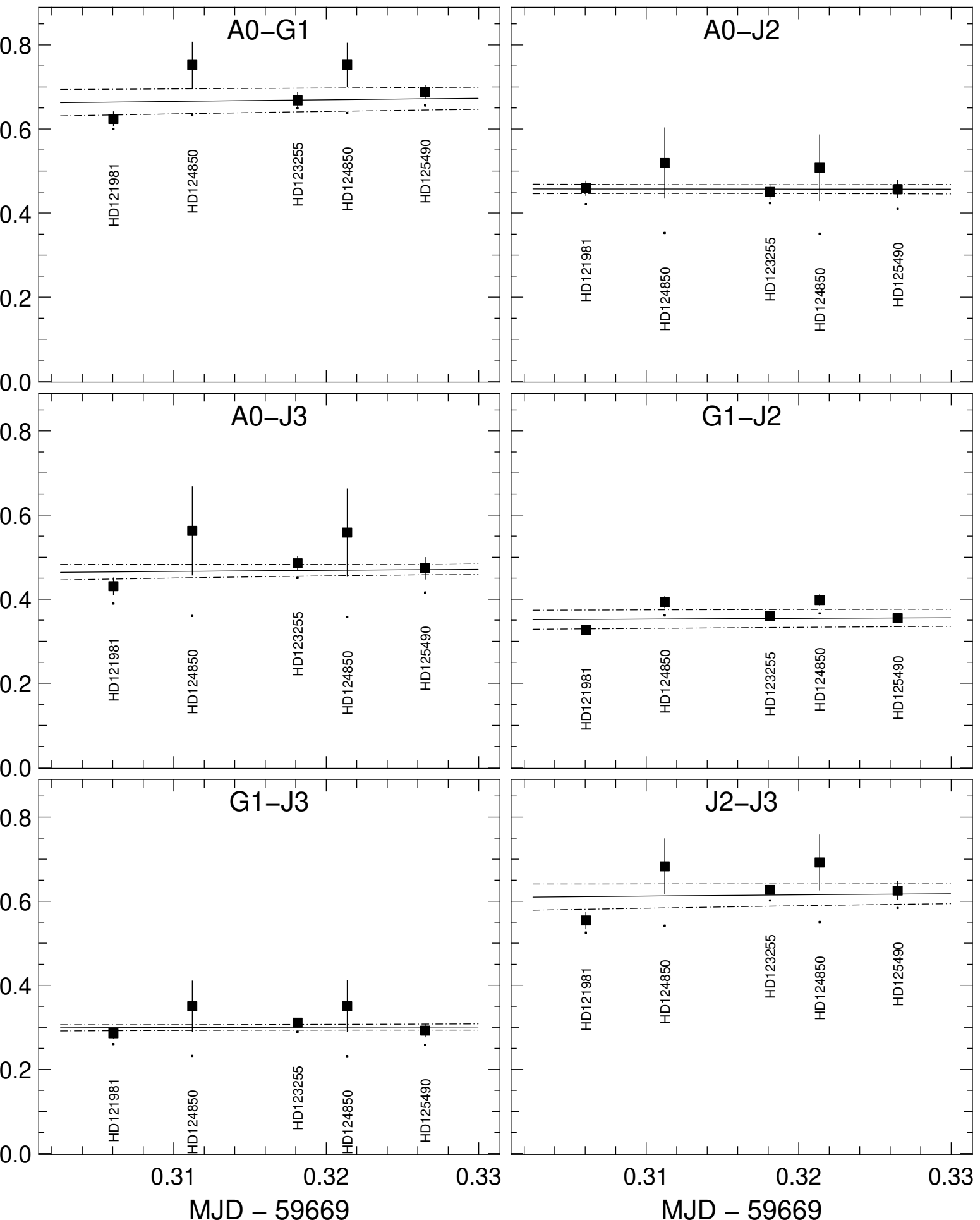
Transfer-Function vis2 (black) and Scientific vis2 (colors) averaged in the range [1.773, 1.773]\mu\text{m}
